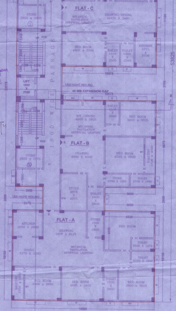
TYPICAL FLOOR PLAN (1st to 5th FLOOR) SCALE - 1:100
