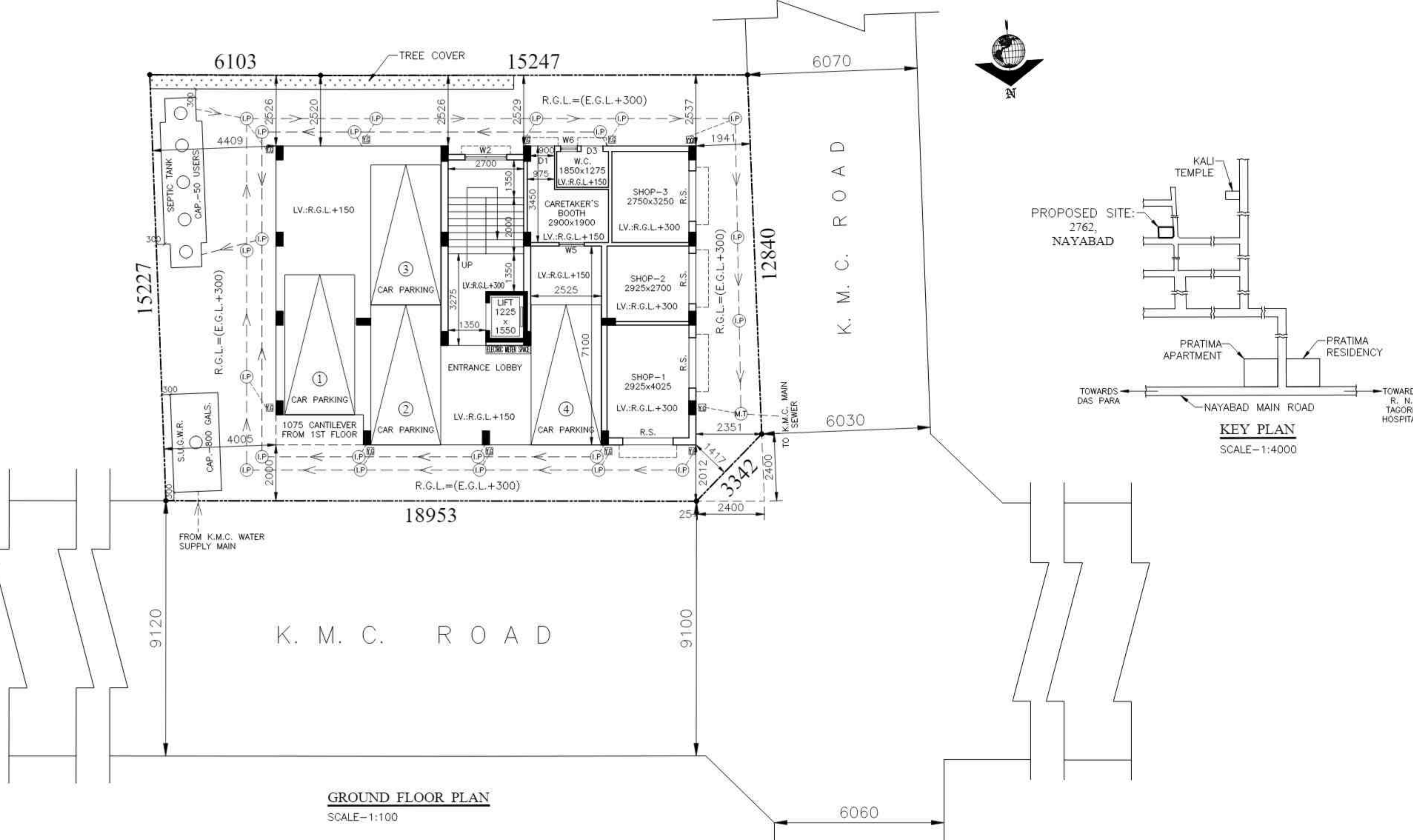
GROUND FLOOR PLAN SCALE-1:100
