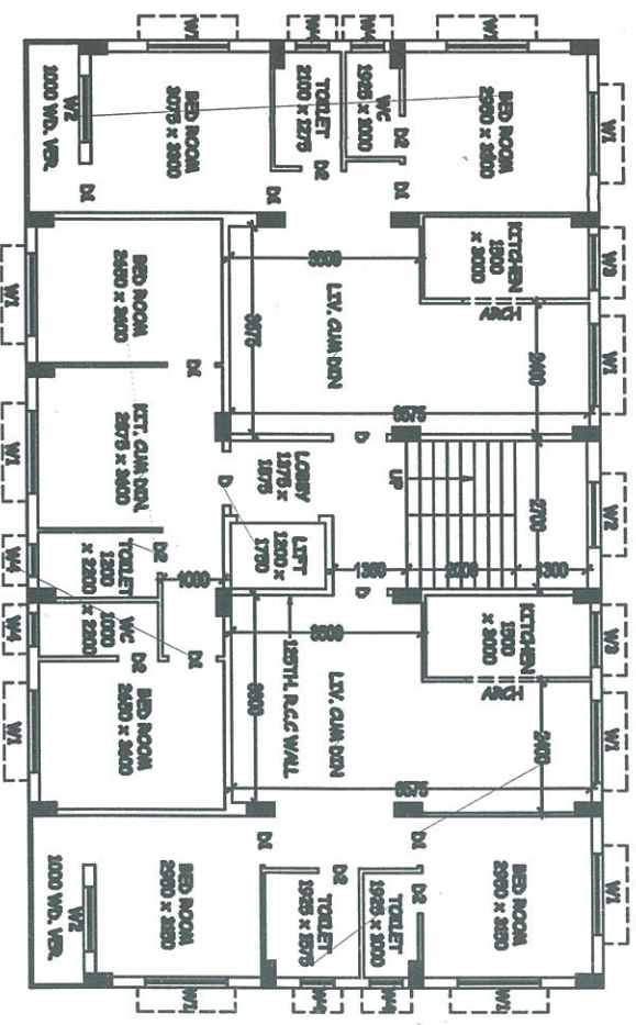
TYPICAL FLOOR PLAN (SECOND & THIRD FLOOR)
