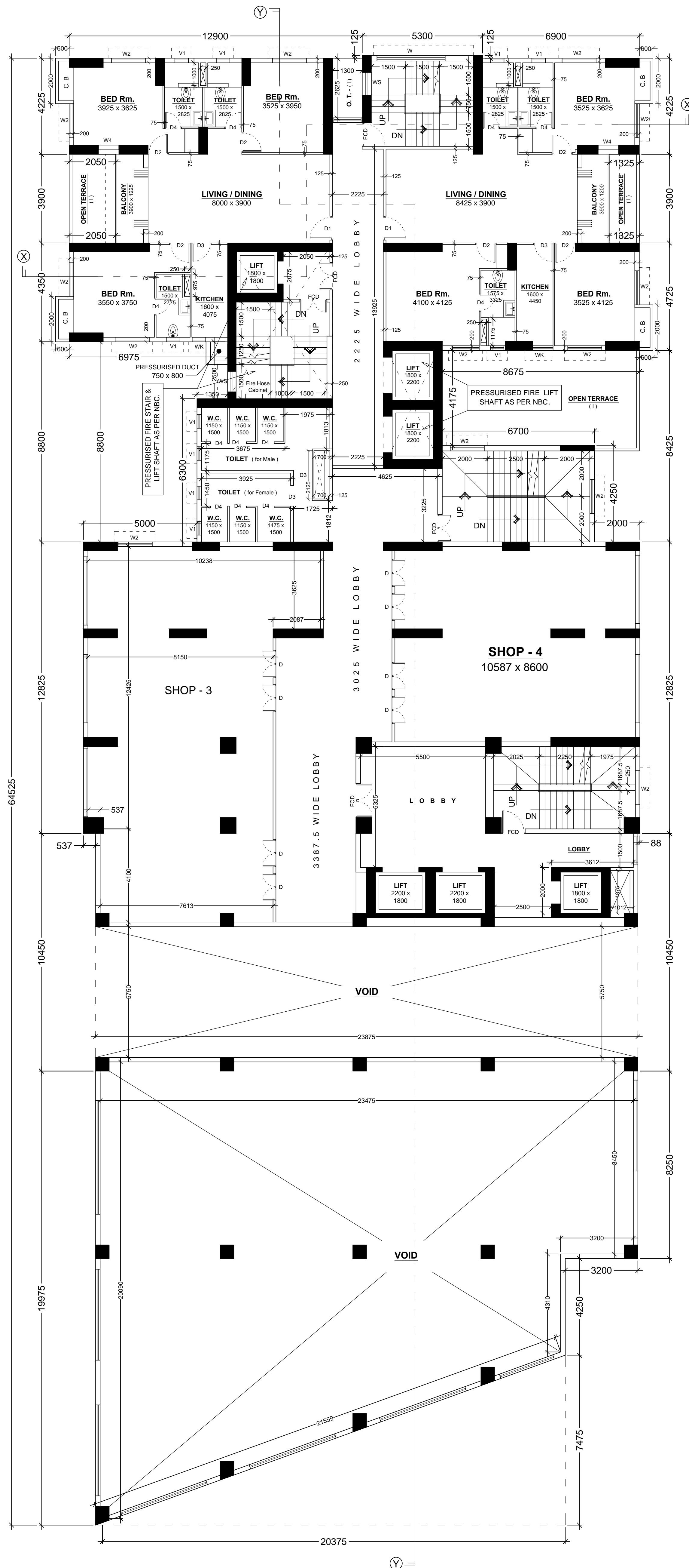
1ST. FLOOR PLAN (SCALE = 1 : 100)
