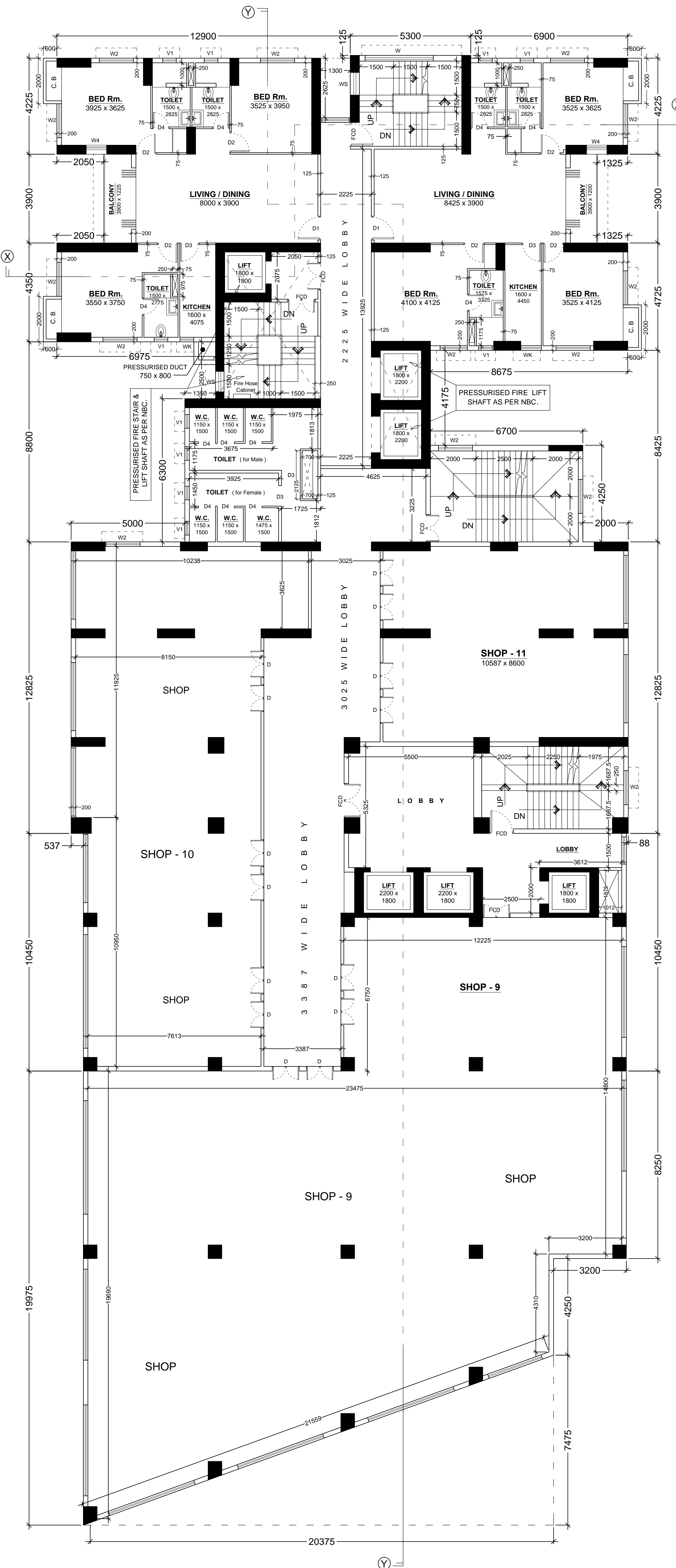
3RD. FLOOR PLAN (SCALE = 1 : 100)
