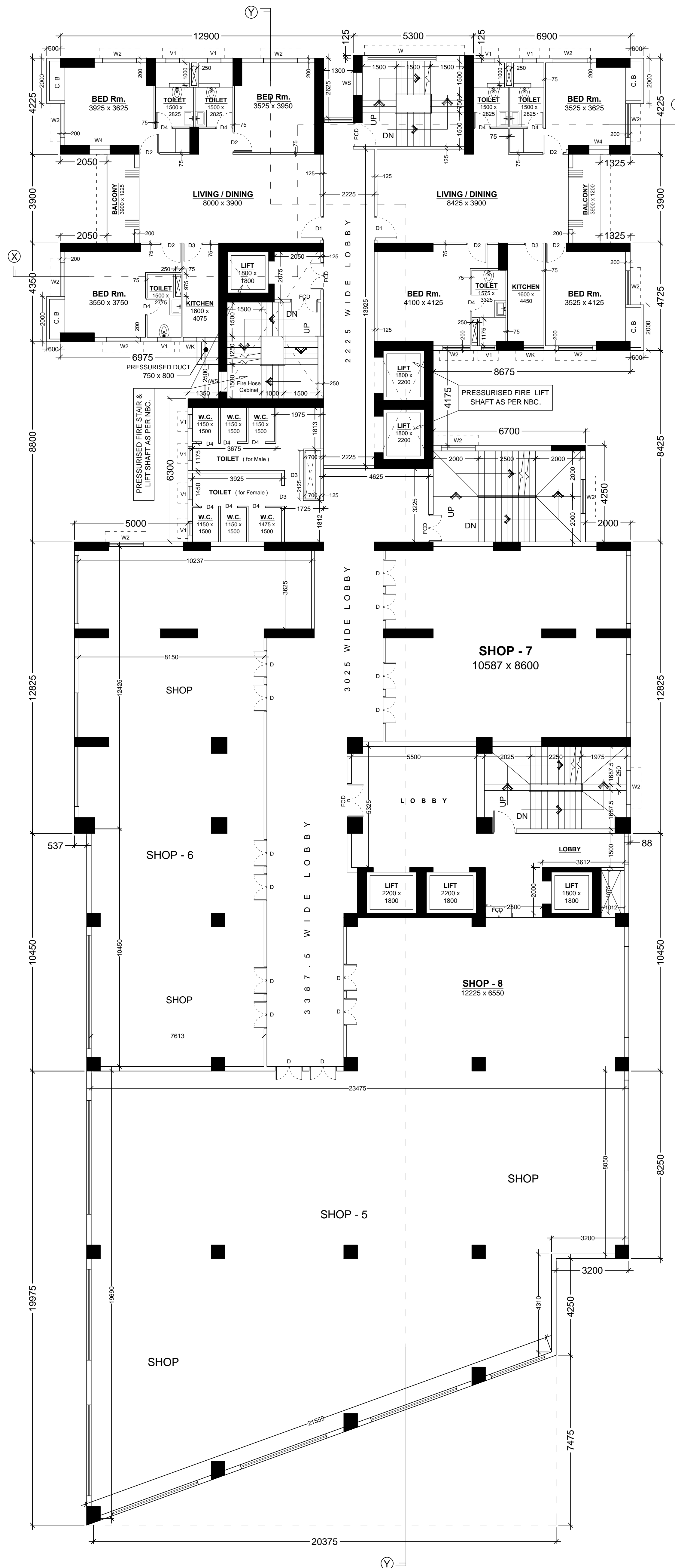
2ND. FLOOR PLAN (SCALE = 1 : 100)
