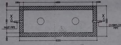
PLAN OF U.S.W.R. (CAPACITY - 2500 Gal.)
