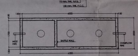
PLAN AND SECTION OF UNDER GROUND FIRE FIGHTING WATER RESERVOIR (CAPACITY - 4500 Gal.)
