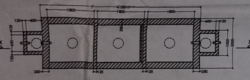
PLAN AND SECTION OF SEPTIC TANK FOR 80 USERS
