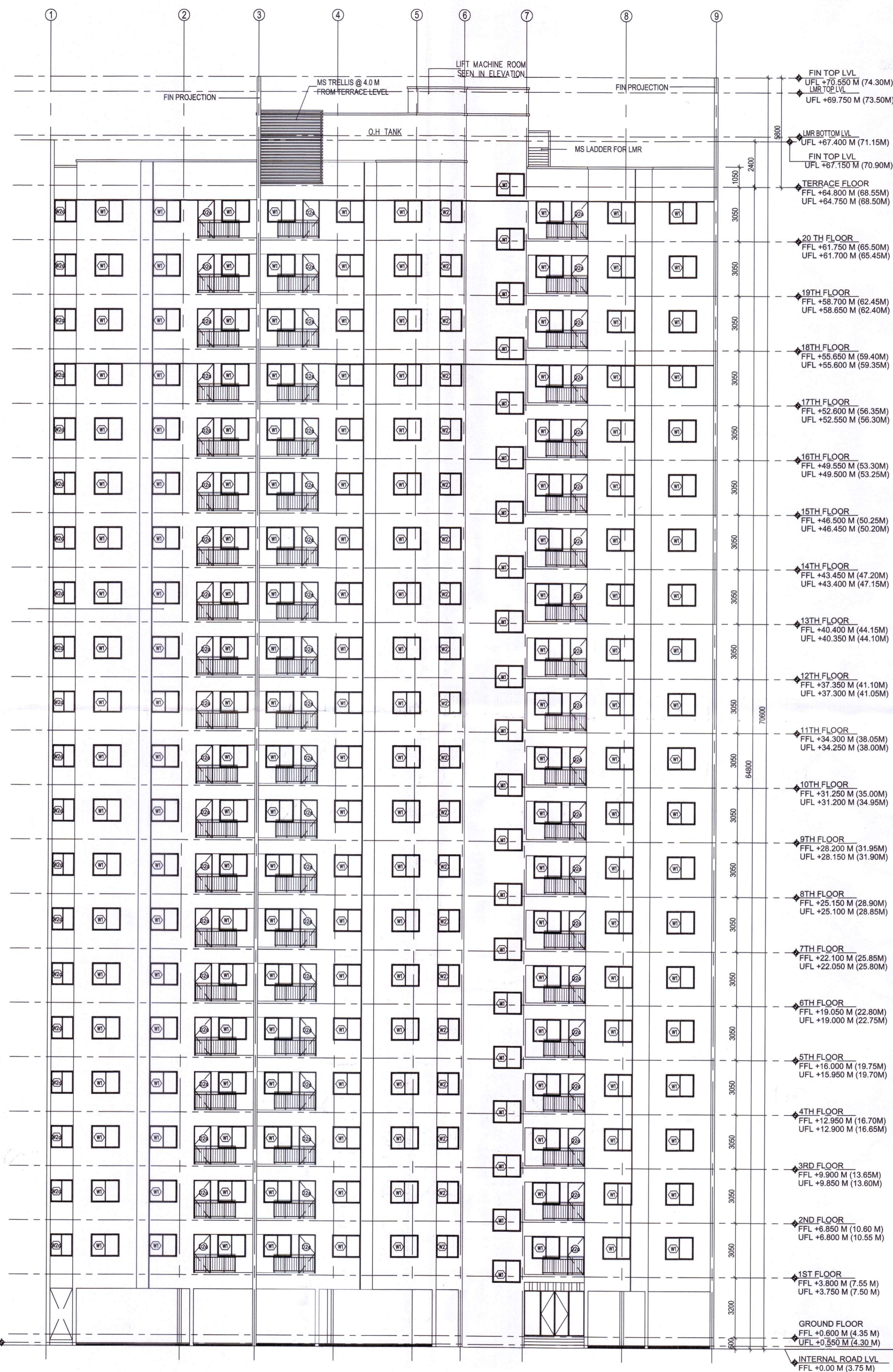
'A' SIDE ELEVATION SCALE 1:125
