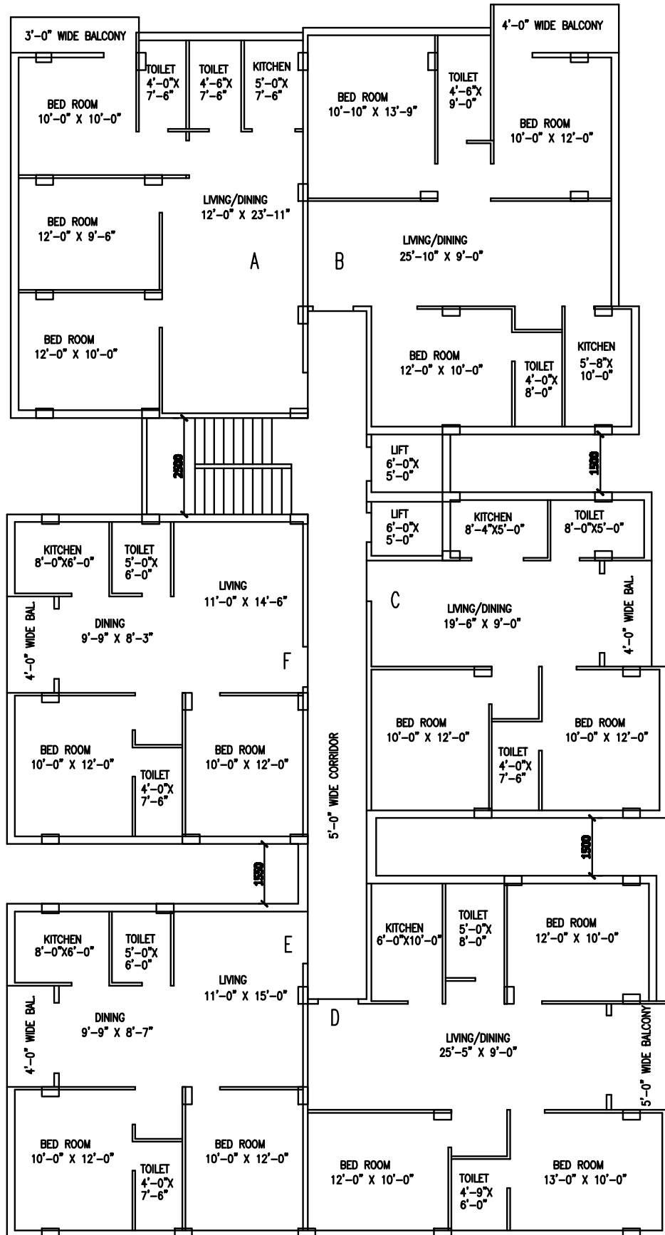
TYP.(1ST-4TH) FLOOR PLAN
