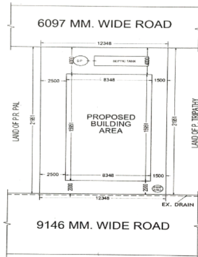
SITE PLAN SCALE- ( 1 : 200 ) DIMENSION ARE IN MM.
