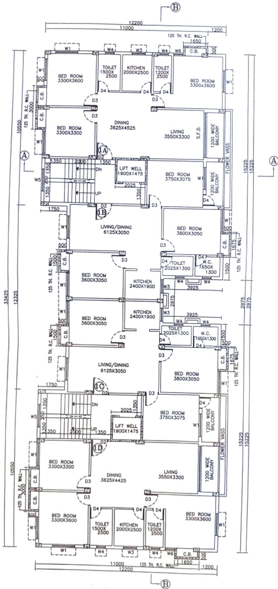
FIRST FLOOR PLAN SCALE-1:100
