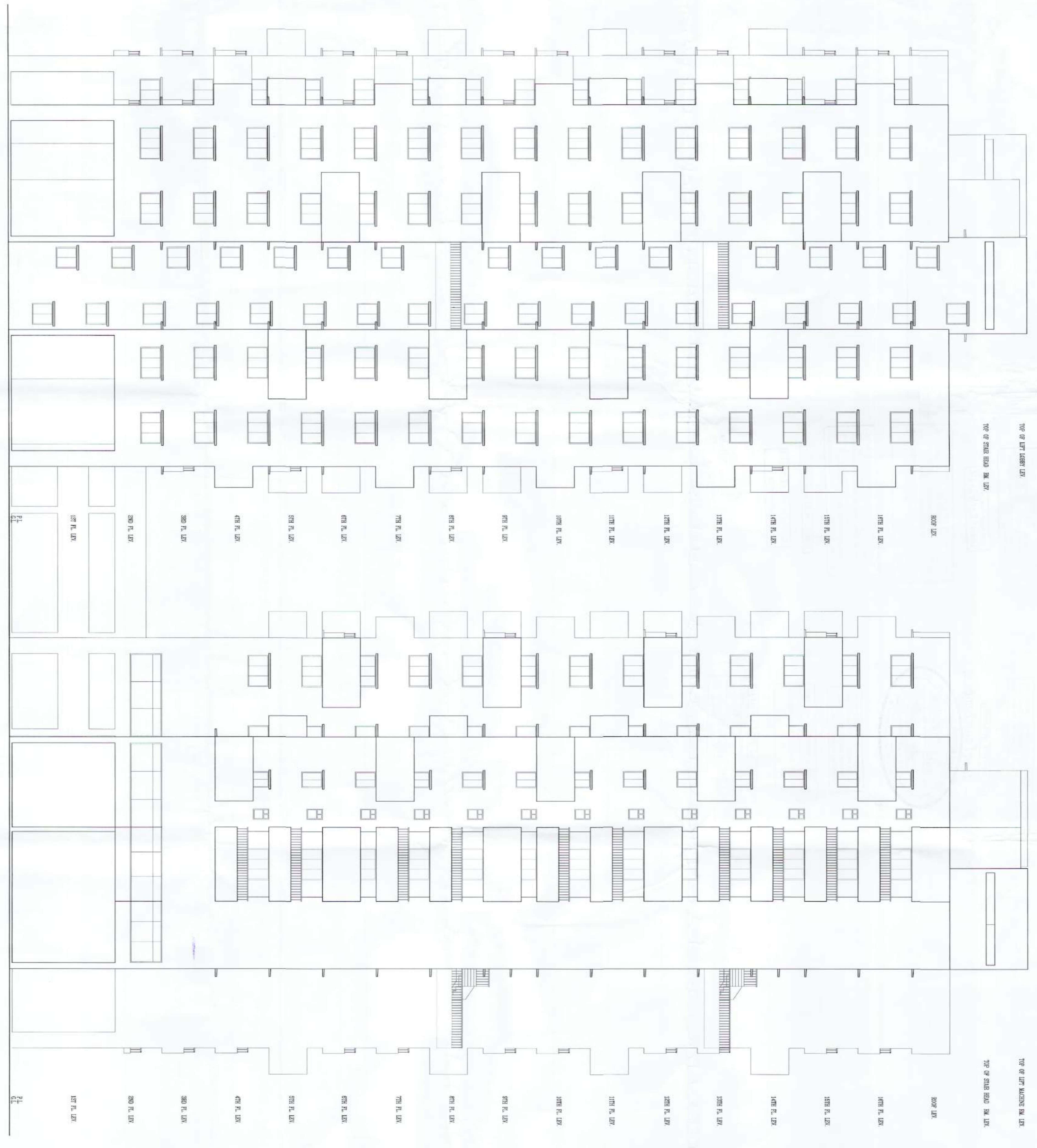
BLOCK-2 FRONT ELEVATION SCALE=1:100
