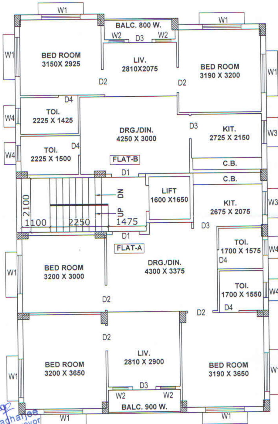
TYPICAL FLOOR PLAN (1ST TO 4TH) 71, BAGUIATI 4TH. LANE.
