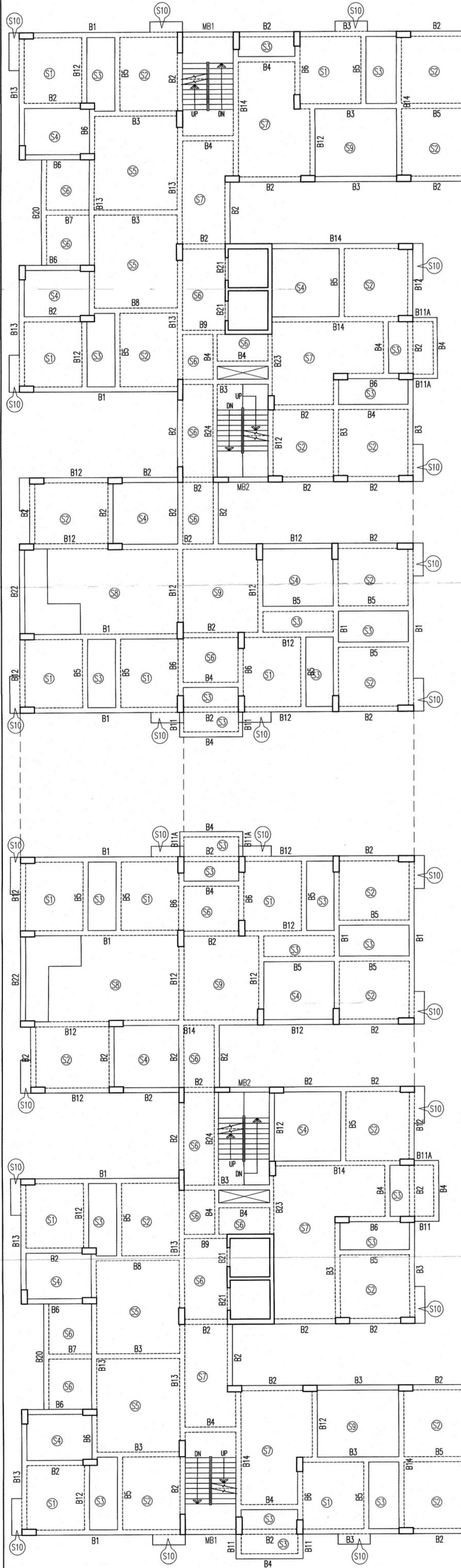
6TH & 9TH FLOOR BEAM LAYOUT
