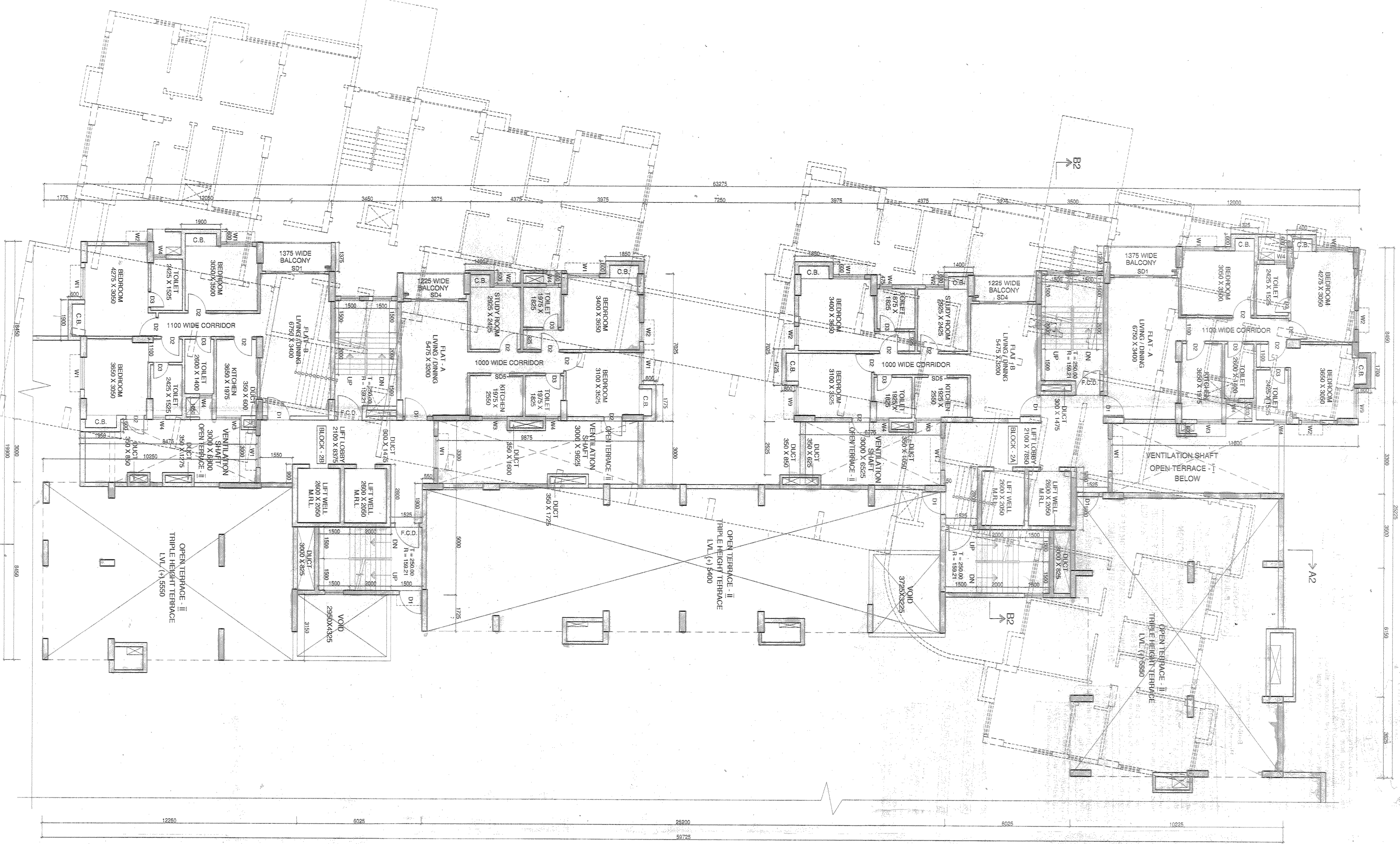
2ND FLOOR PLAN
