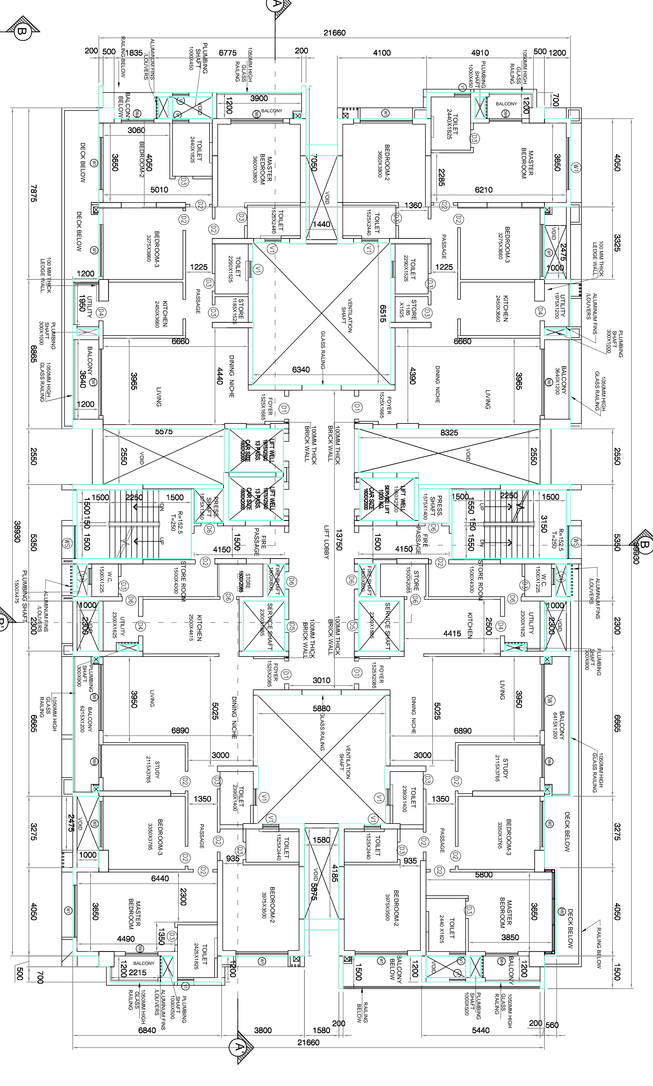
FLOOR PLAN(LOWER LEVEL) 11TH & 21ST FLOOR
