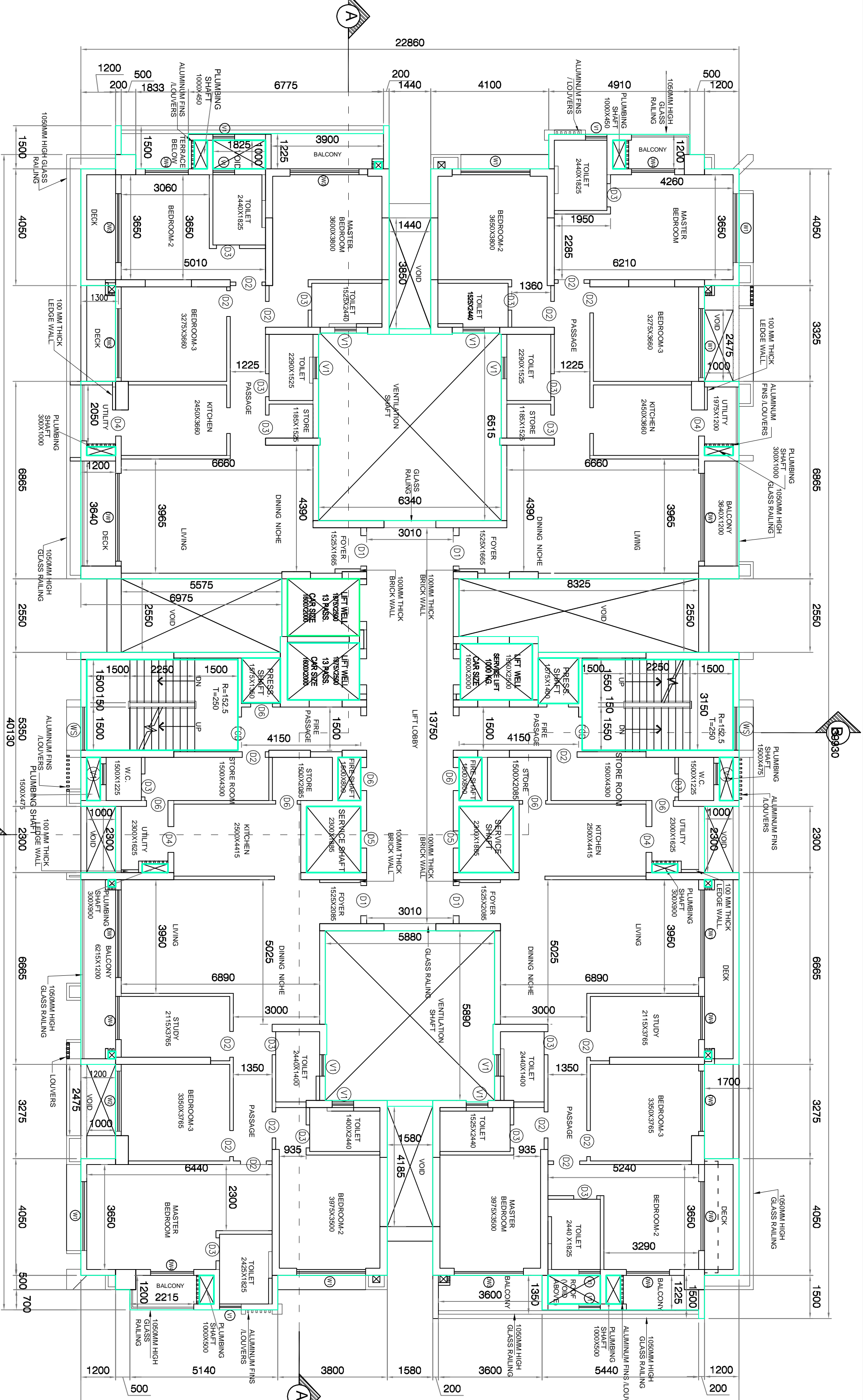
FLOOR PLAN(LOWER LEVEL) 10TH & 20TH FLOOR
