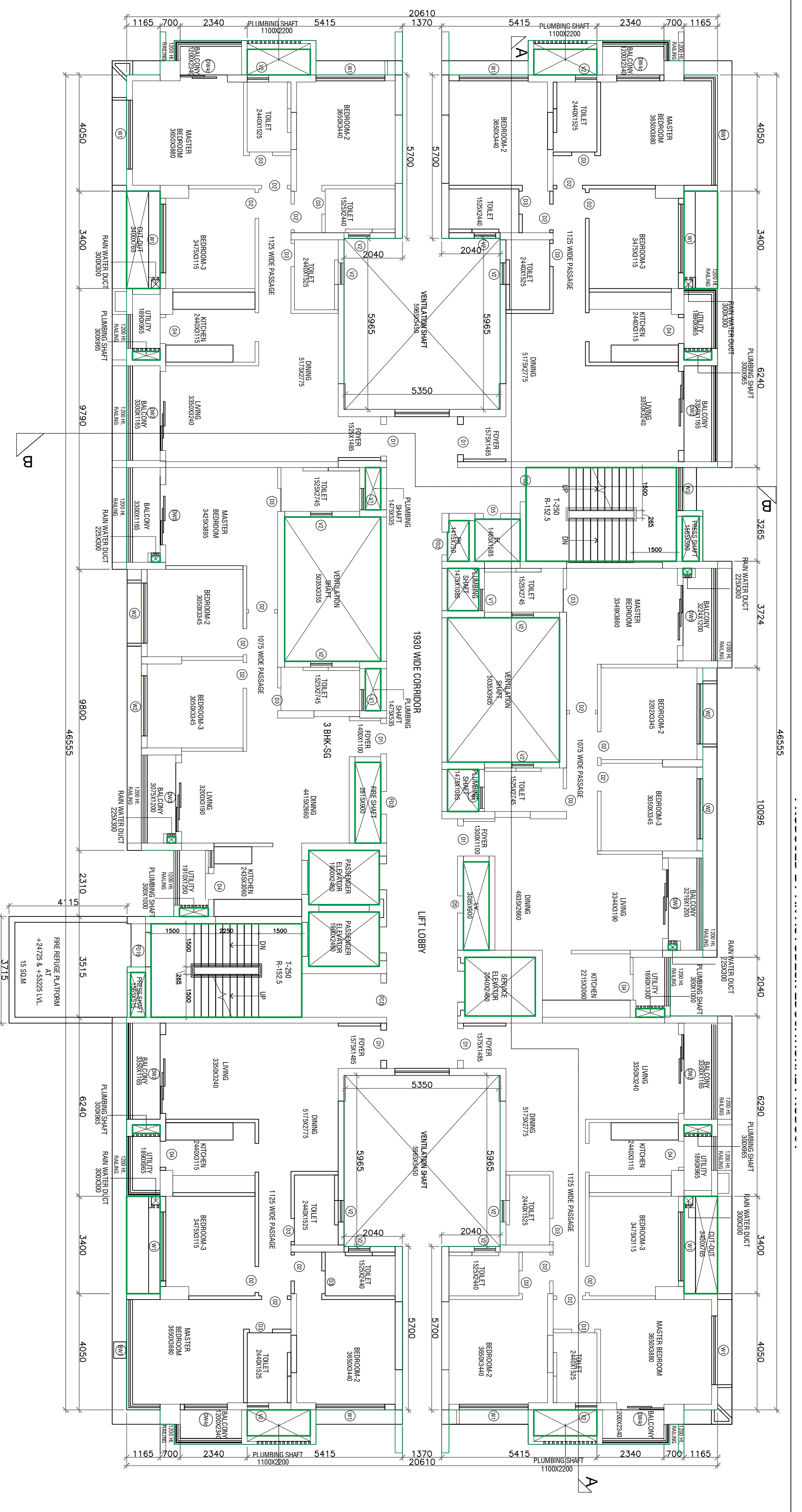
6TH AND 16TH FLOOR PLAN (FIRE REFUGE FLOOR)
