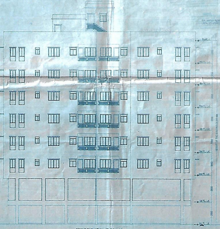
FRONT ELEVATION (BLOCK 1) SCALE: 1:100
