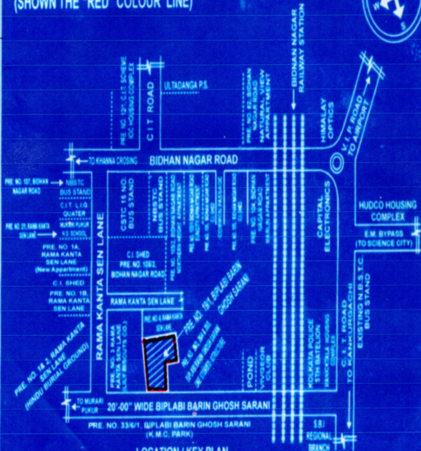
LOCATION / KEY PLAN SCALE- 1:4000
