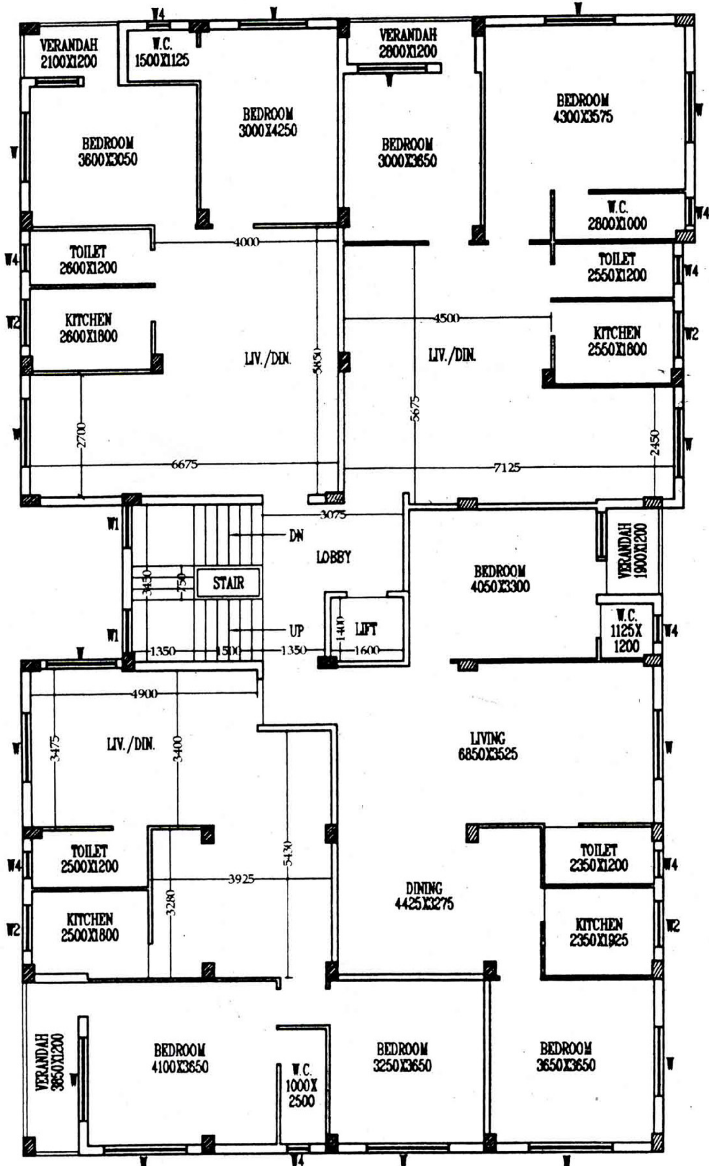
TYPICAL FLOOR PLAN OF BLOCK -B
