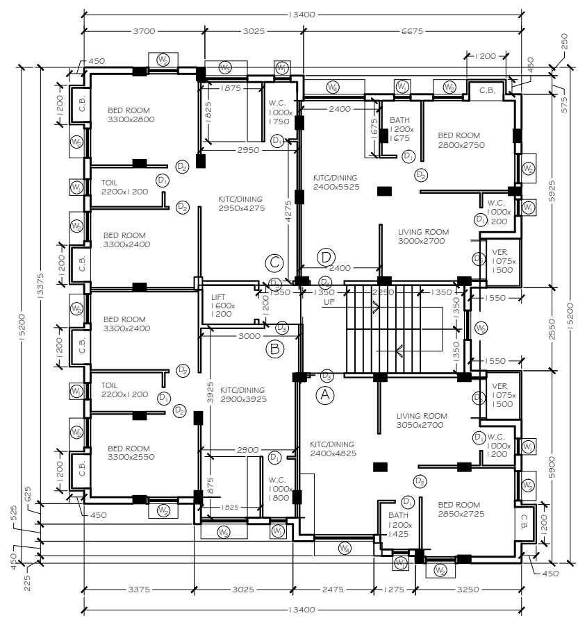
IST, 2ND, 3RD & 4TH FL. PLAN
