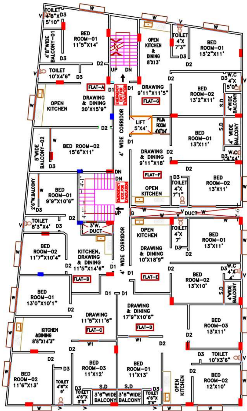
PROPOSED FIRST FLOOR PLAN SCALE 1:96
