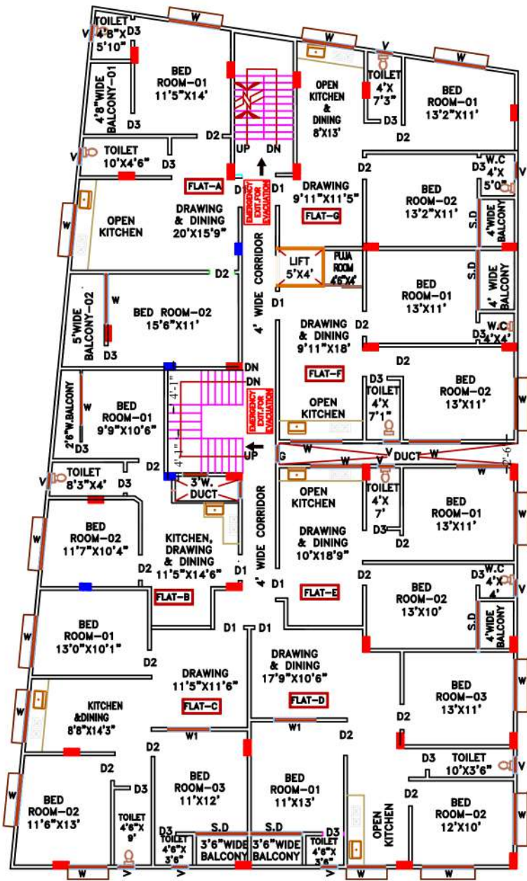
PROPOSED THIRD FLOOR PLAN SCALE 1:96
