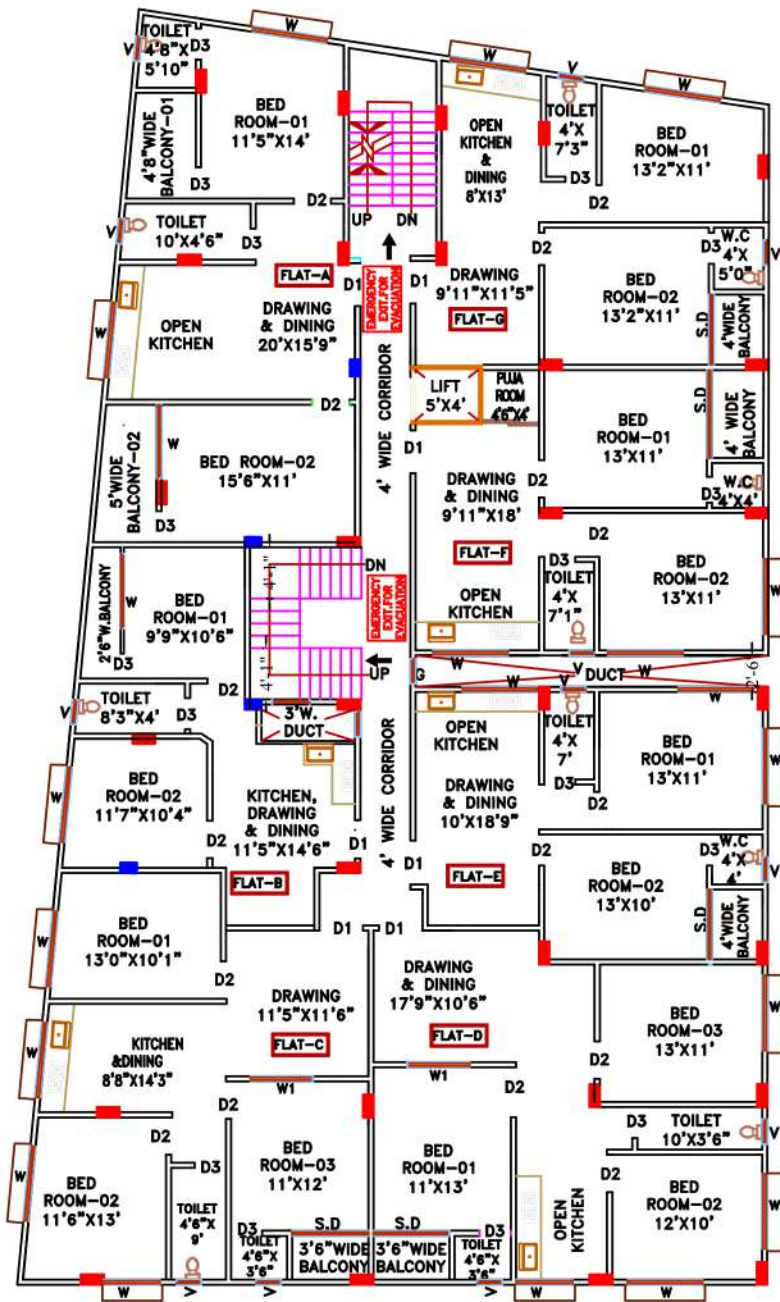
PROPOSED SECOND FLOOR PLAN SCALE 1:96
