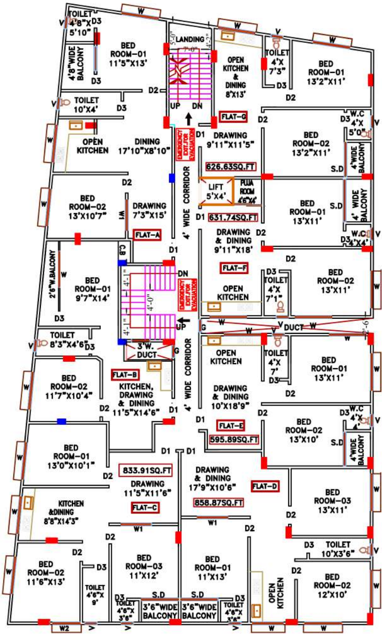
PROPOSED FOURTH FLOOR PLAN SCALE 1:96
