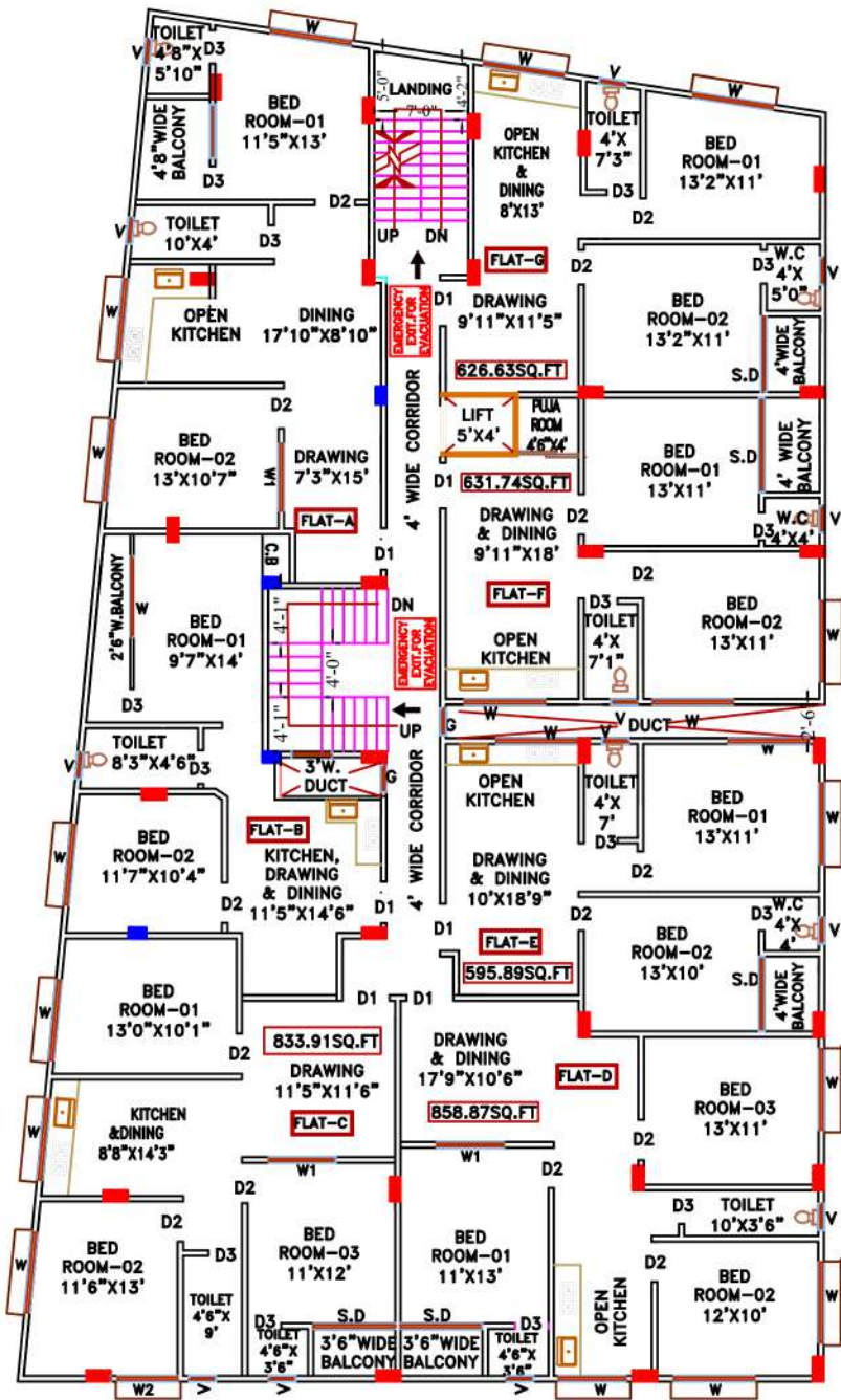
PROPOSED FIFTH FLOOR PLAN SCALE 1:96
