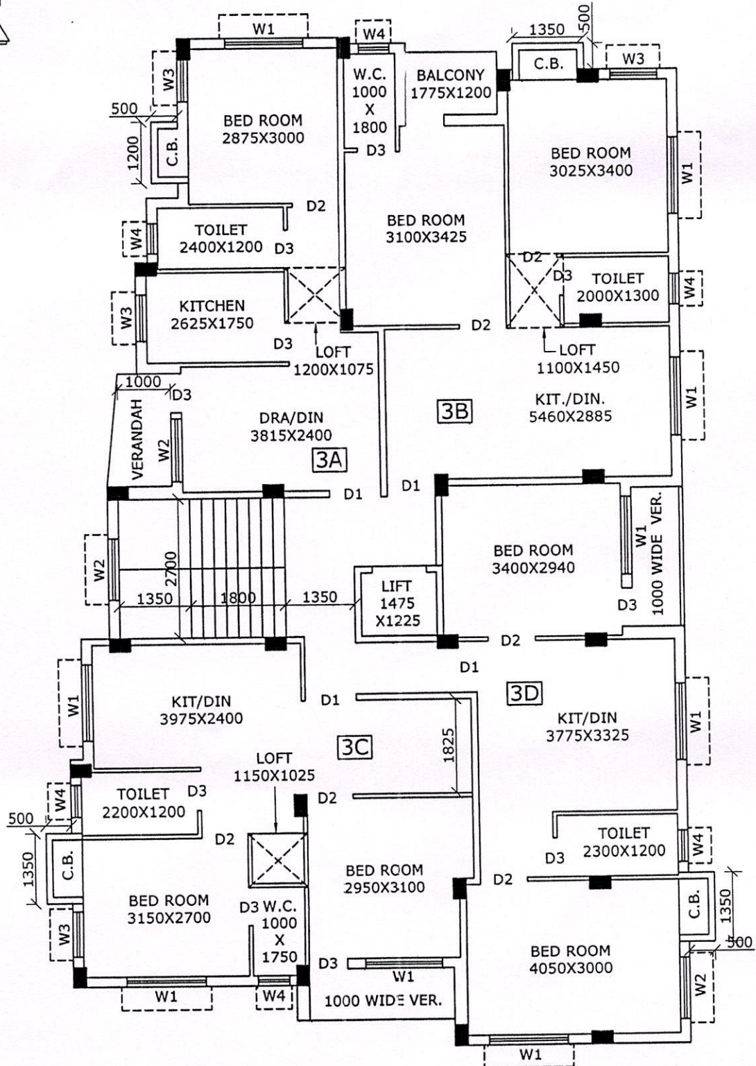
3RD FLOOR PLAN
