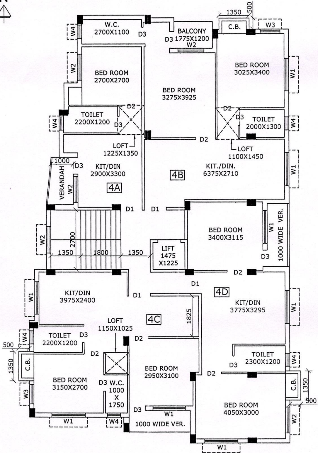
4TH FLOOR PLAN
