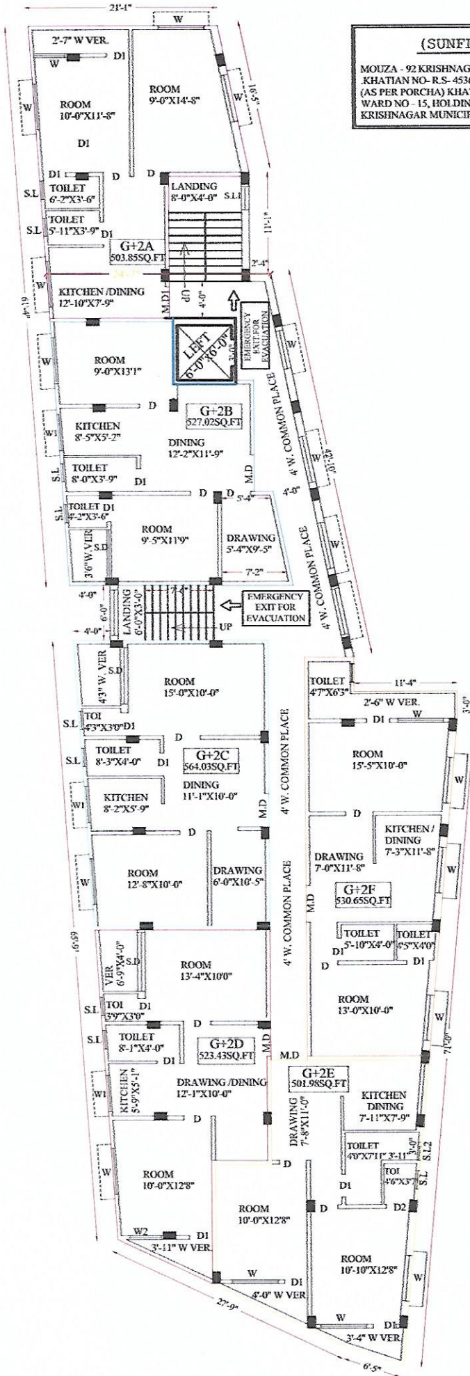
TOTAL 6 FLATS IN SECOND FLOOR PLAN SCALE - 1:96
