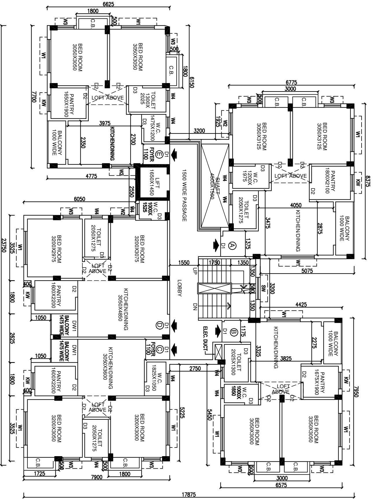
TYPICAL FLOOR PLAN (1ST TO 3RD FLOOR)
