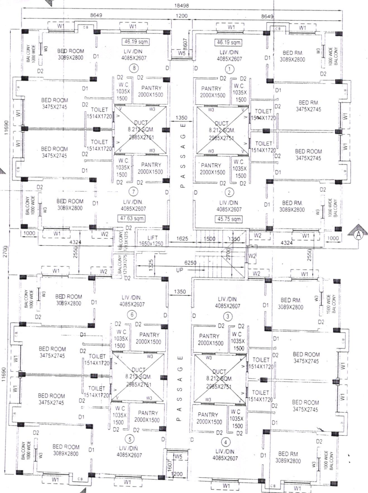
TYPICAL FLOOR PLAN (BLOCK-1)
