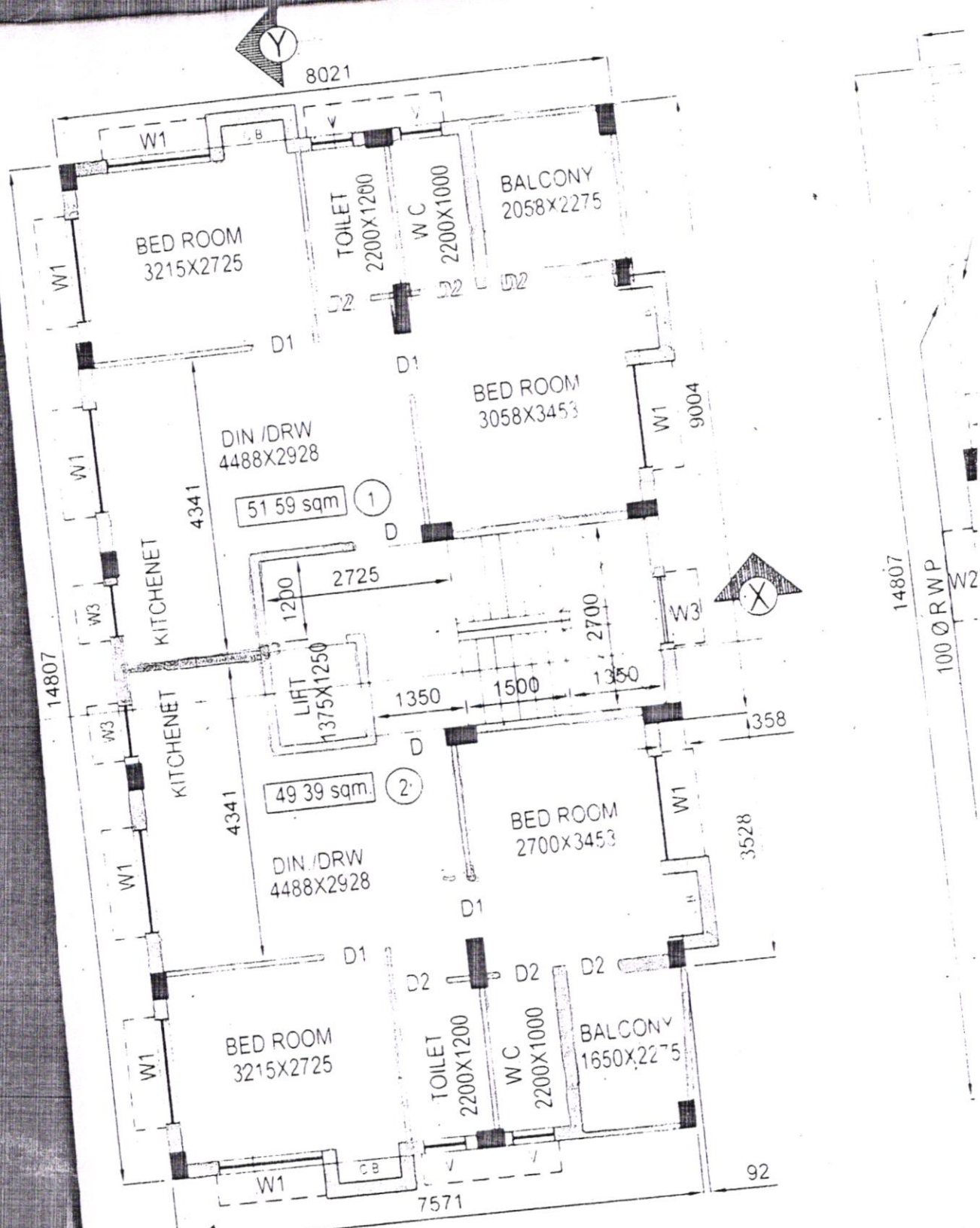
TYPICAL FLOOR PLAN (BLOCK-2)
