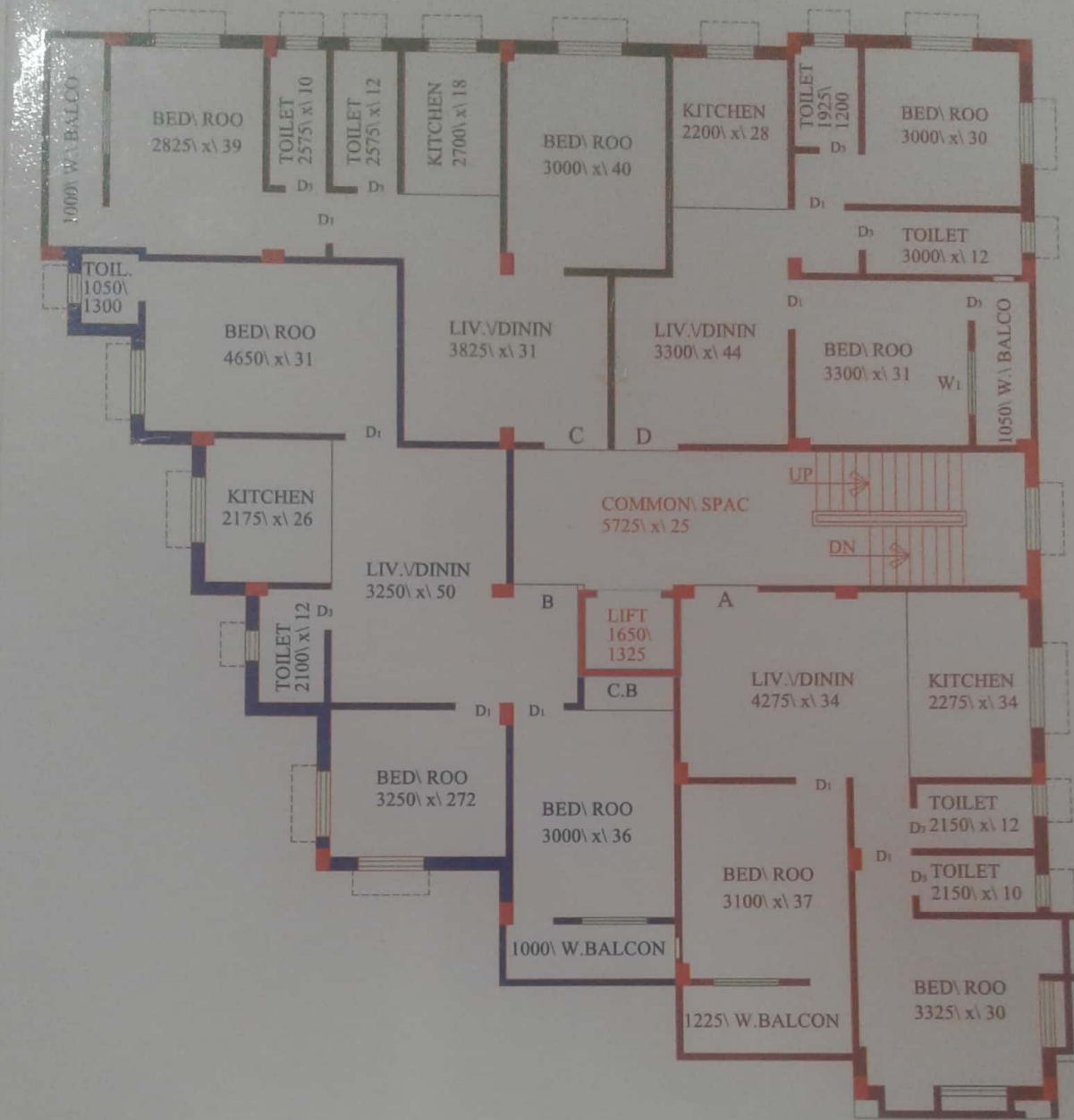
TYPICAL FLOOR PLAN = ( 2ND, 3RD )
