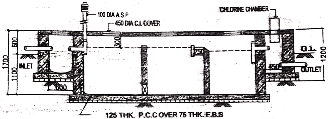
SECTION X-X
