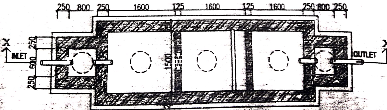
PLAN OF SEPTIC TANK (75 USERS)
