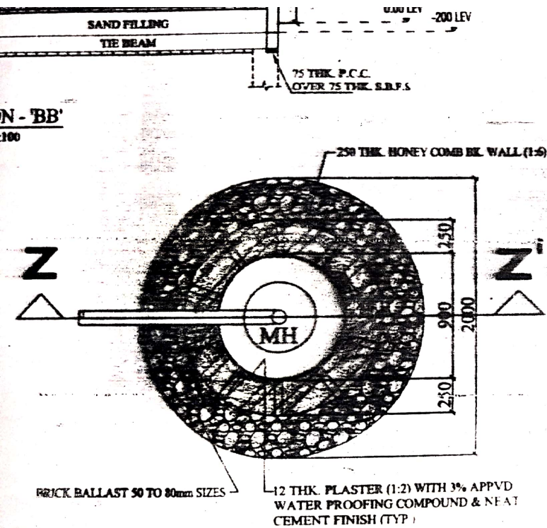
TYP. G.A. PLAN OF SOAK PIT
