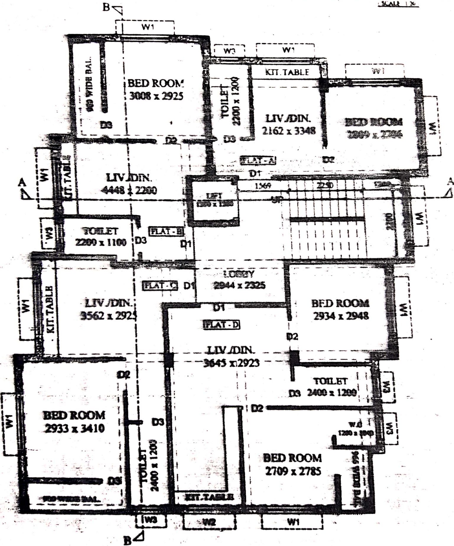
PROP. TYP. (1ST-3RD) FLOOR PLAN SCALE:-1:100
