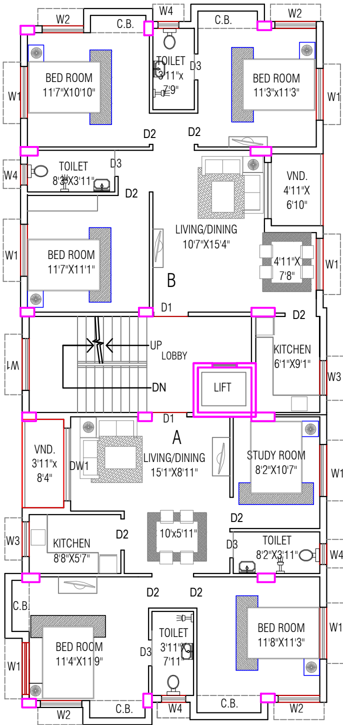
(1st.,2nd,3rd.& 4th. FLOOR PLAN)
