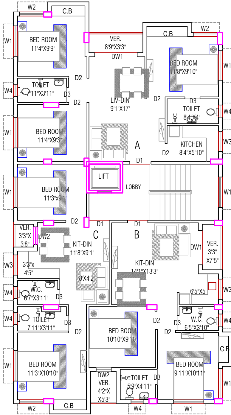
TYPICAL (1ST. TO 4TH.) FLOOR PLAN
