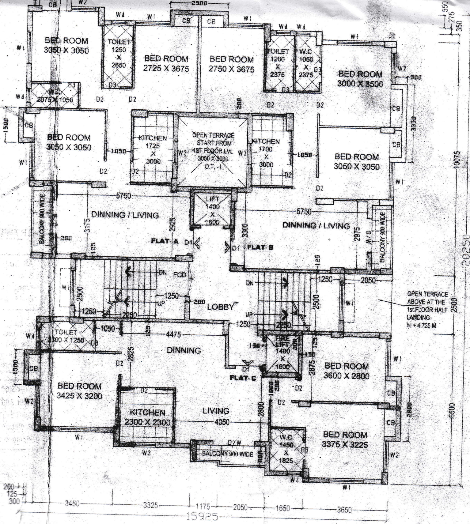
2ND TO 7TH FLOOR PLAN SCALE - 1:100
