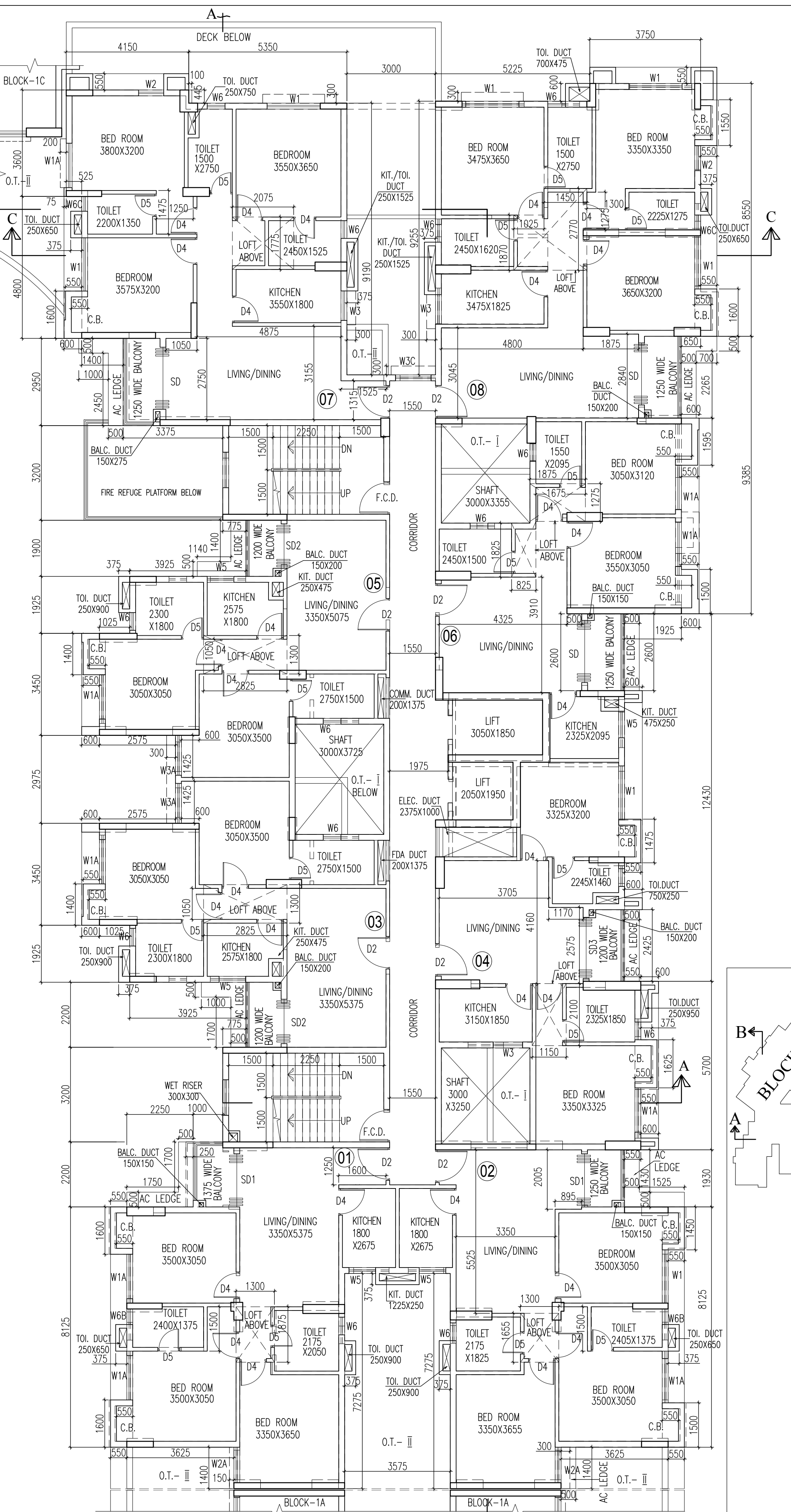
13TH. FLOOR PLAN BLOCK-1B
