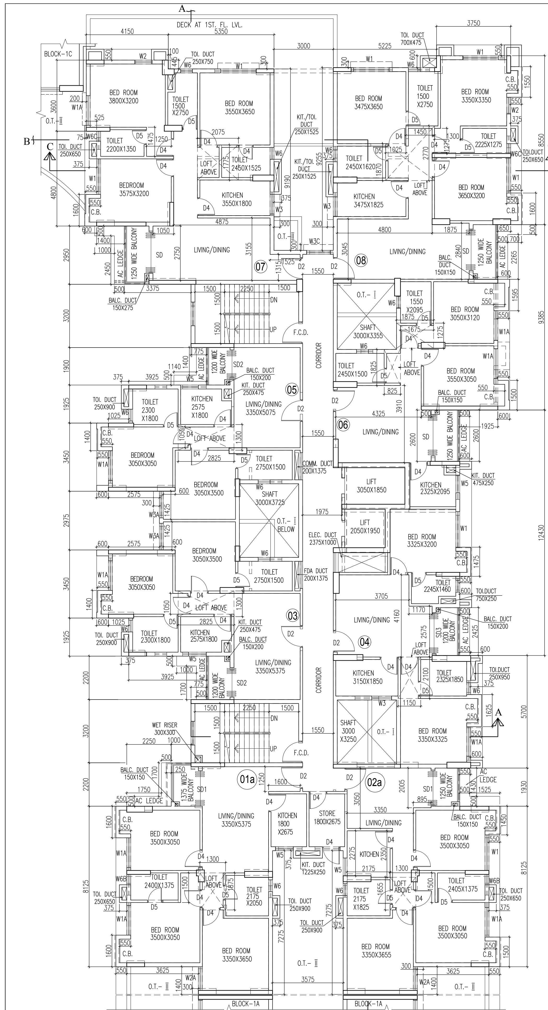
SECOND FLOOR PLAN BLOCK-1B
