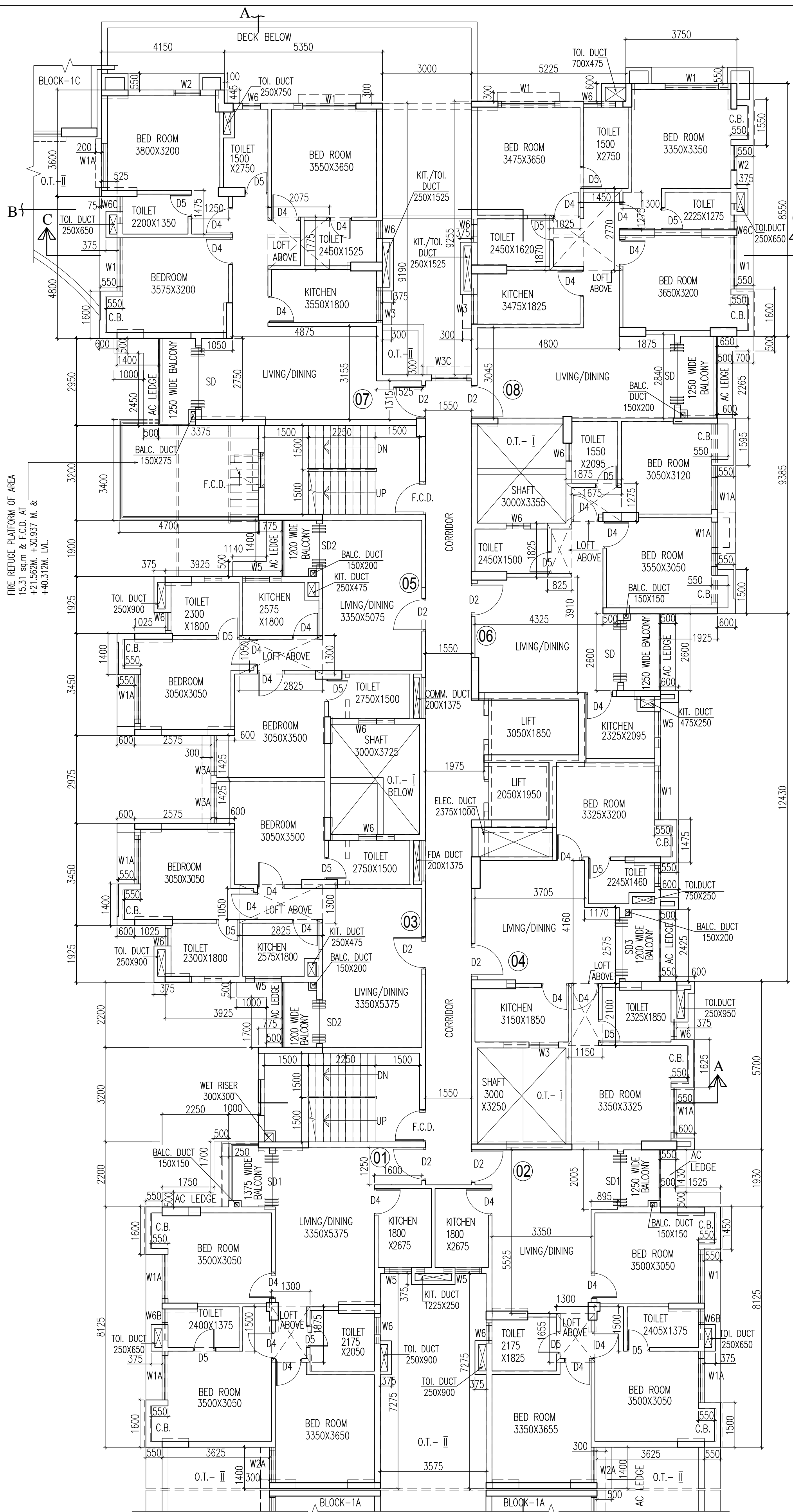
TYPICAL FLOOR (3RD. TO 12TH) PLAN BLOCK-1B
