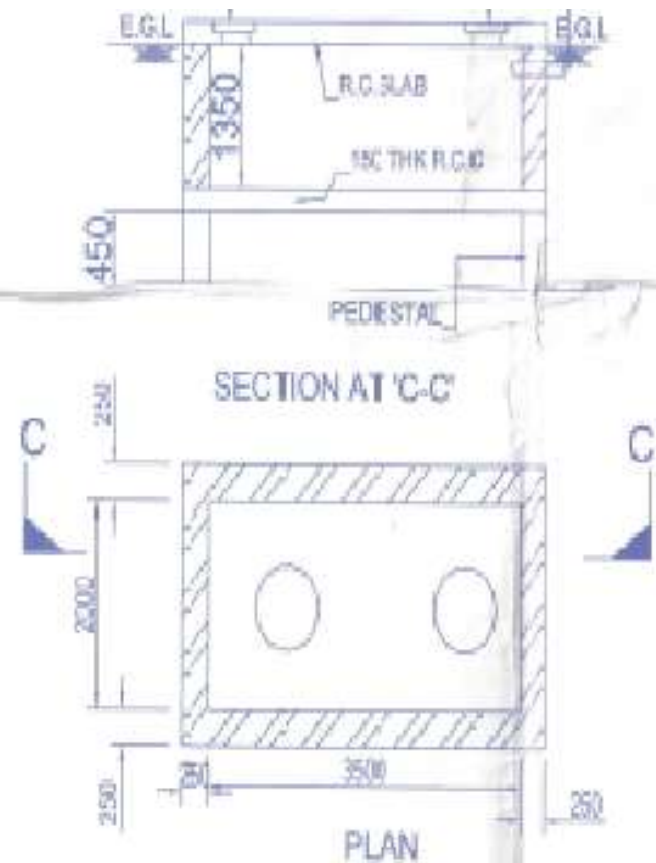
DETAILS OF UNDER GROUND RESERVOIR (CAPACITY - 12000LIT)
