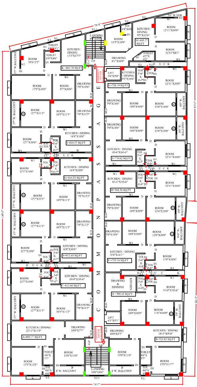
FIFTH FLOOR PLAN SCALE 1:96
