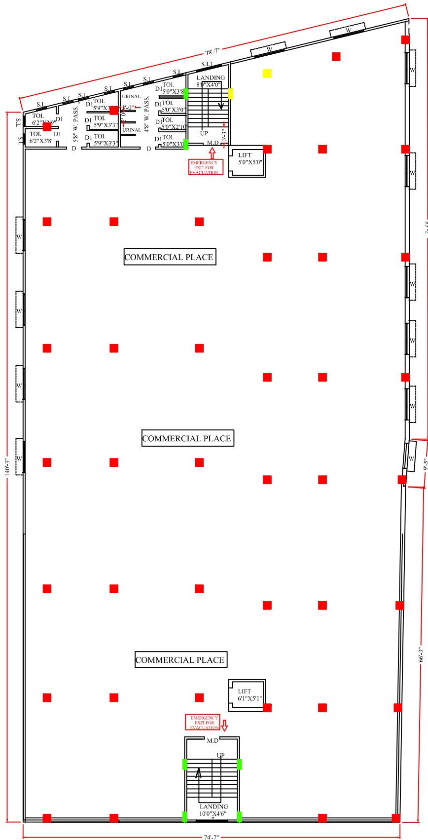
FIRST FLOOR PLAN SCALE 1:96
