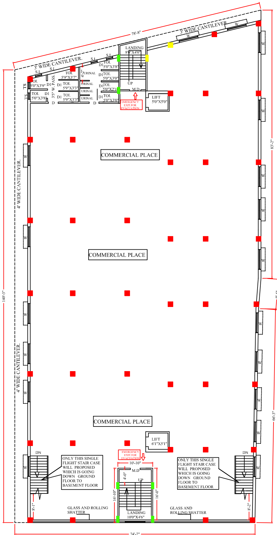
GROUND FLOOR PLAN WITH SITE PLAN SCALE 1:96
