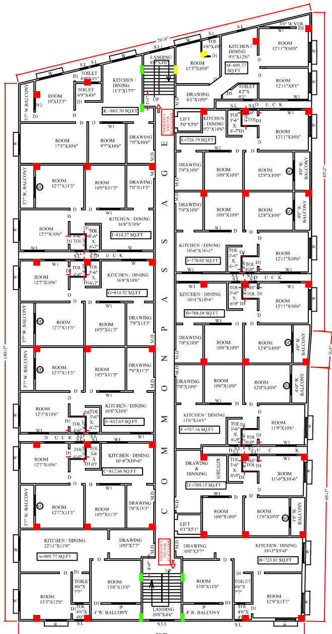
SECOND FLOOR PLAN SCALE 1:96 LV = +19'10"
