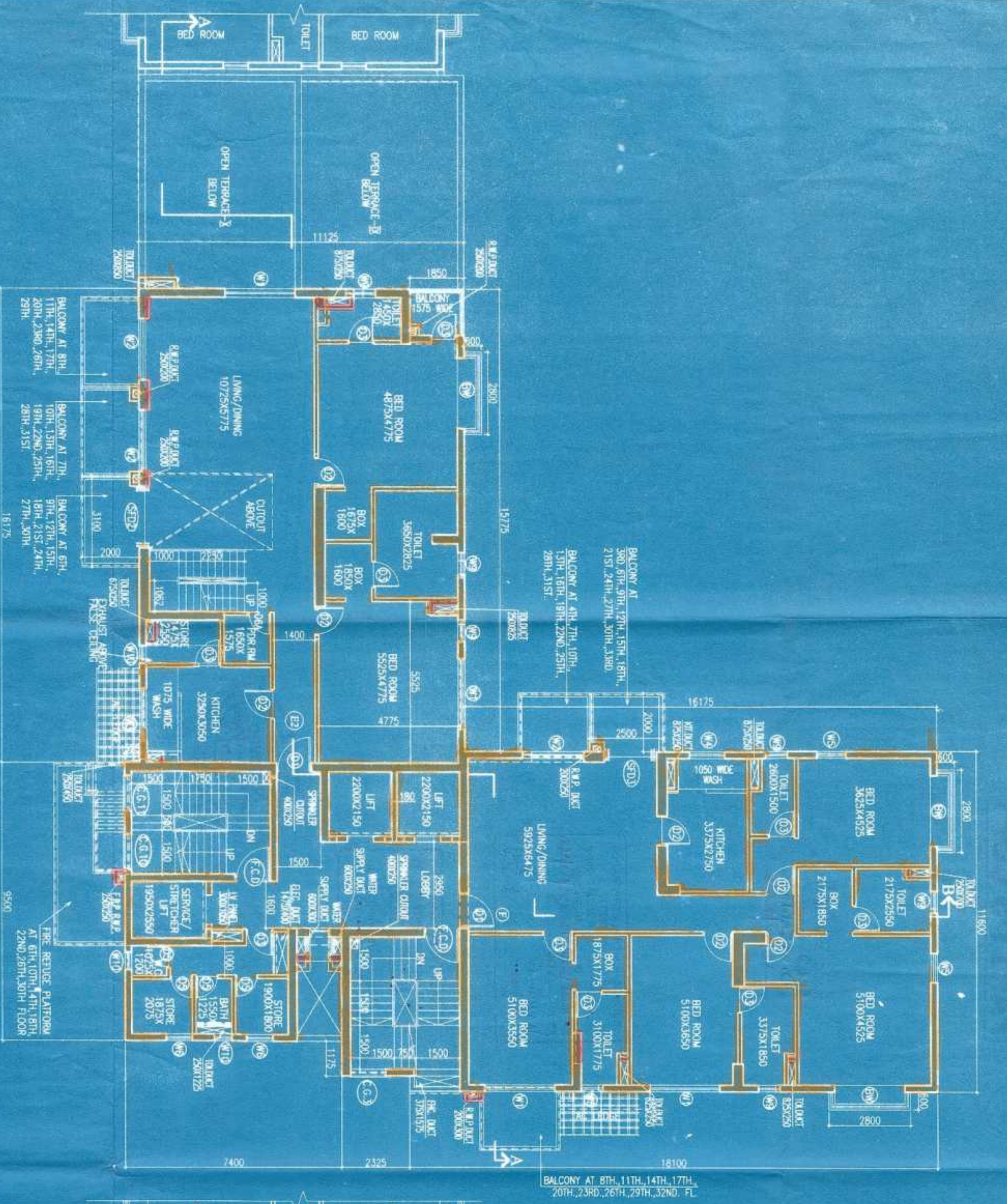
12TH FLOOR PLAN
