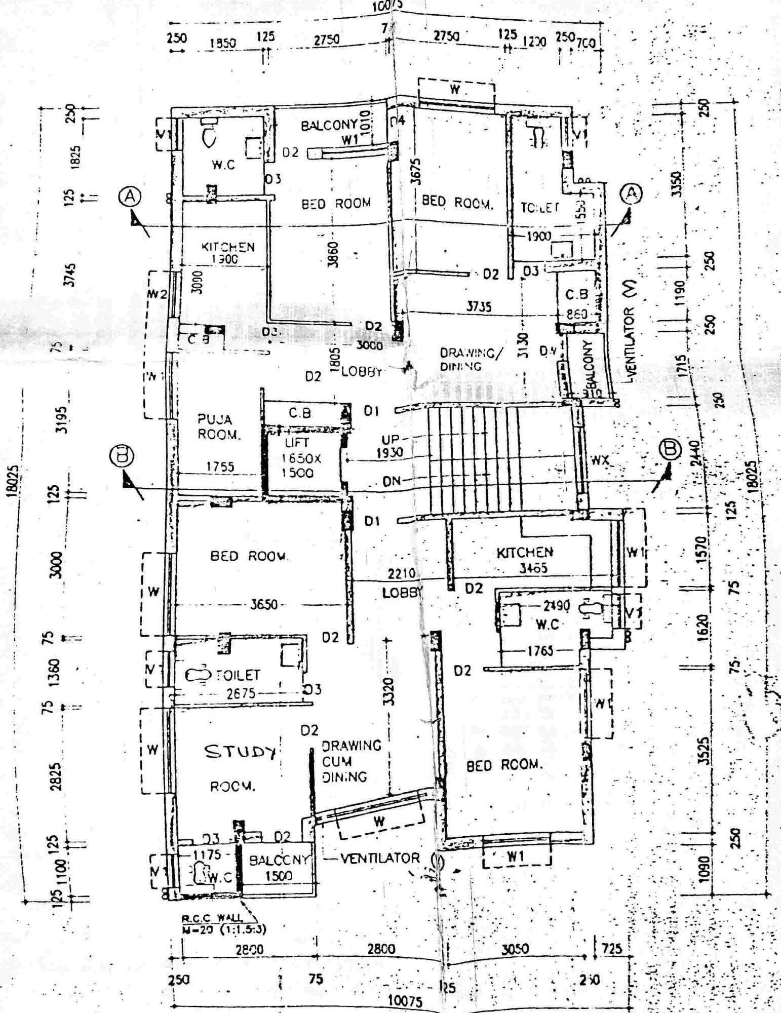
2ND, 3RD, 4TH FLOOR PLAN SCALE - 1:100
