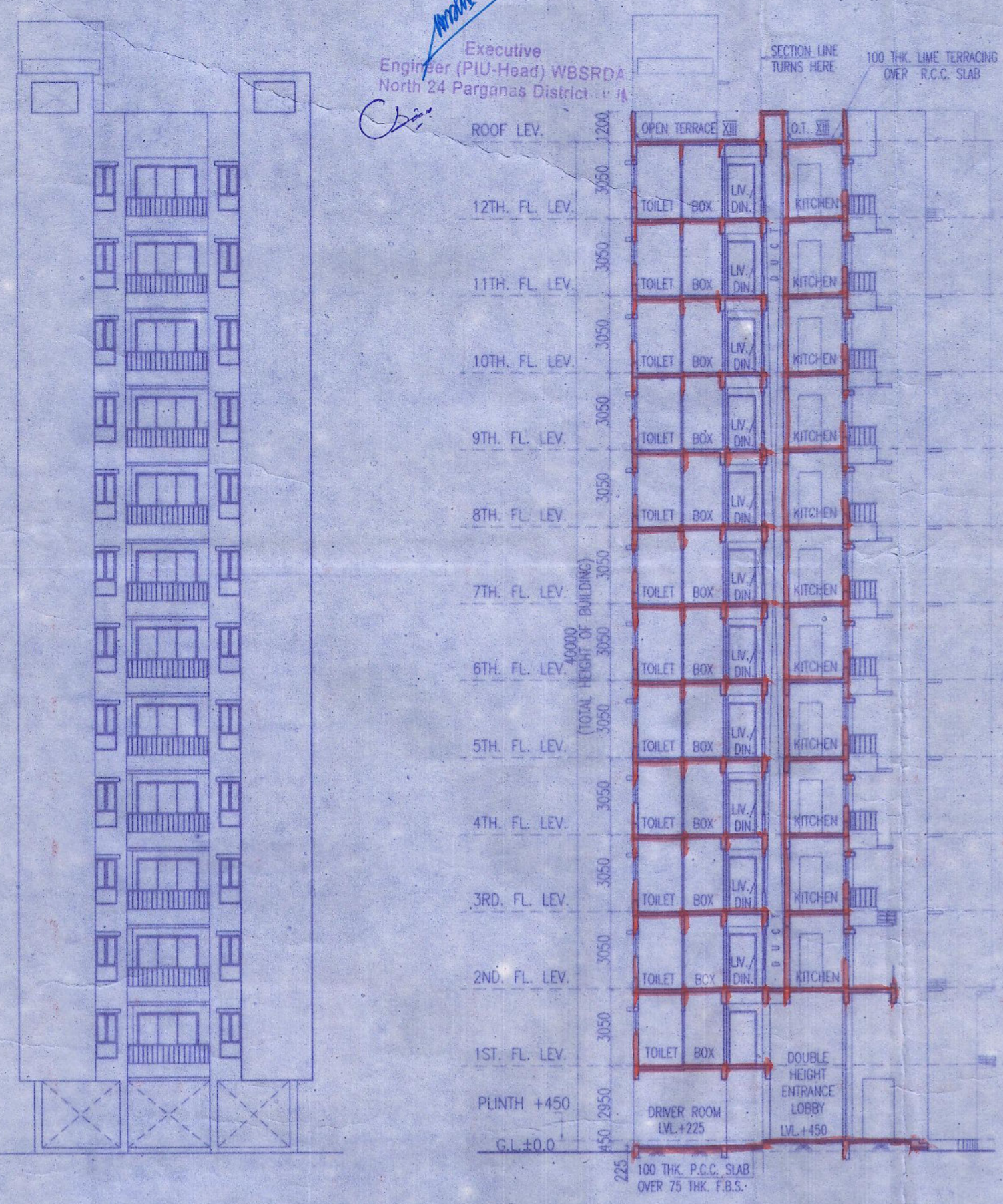
FRONT ELEVATION
