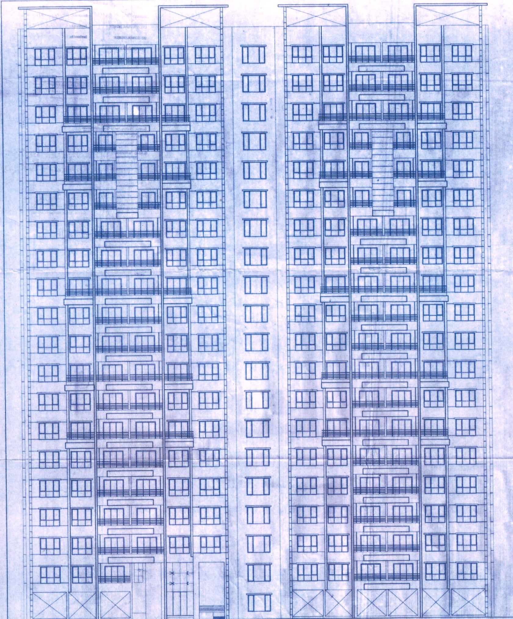
FRONT ELEVATION
