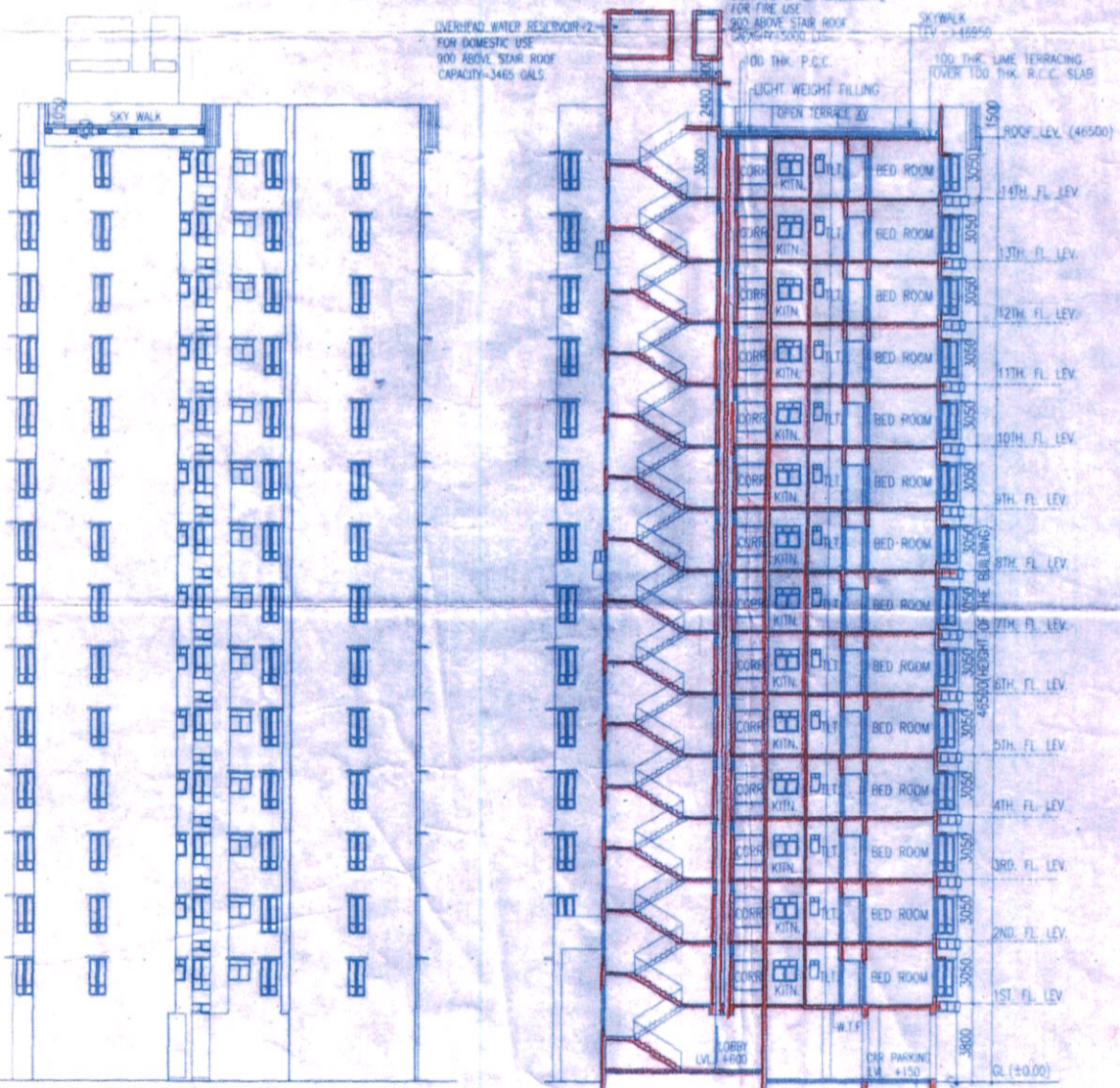
SECTION K-K
