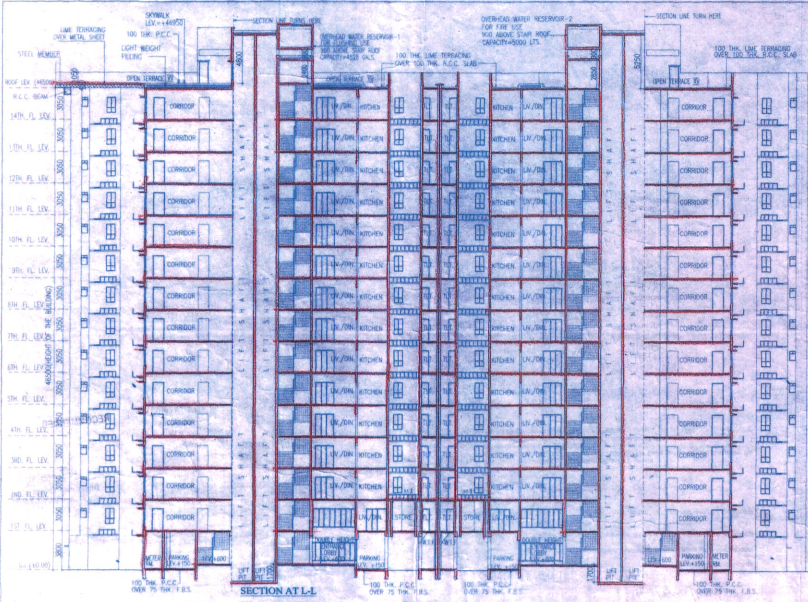
SECTION AT-L-L
