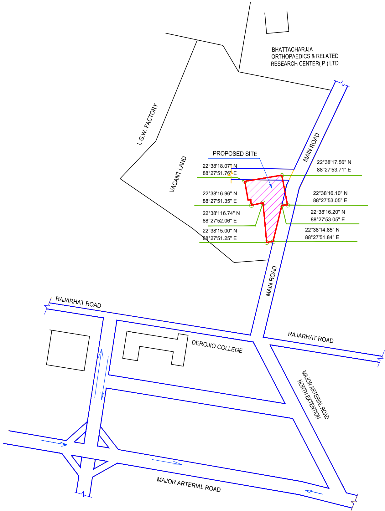
LOCATION PLAN OF UNIMARK SPRINGFIELD PLOT 4 (ELITE 2)
