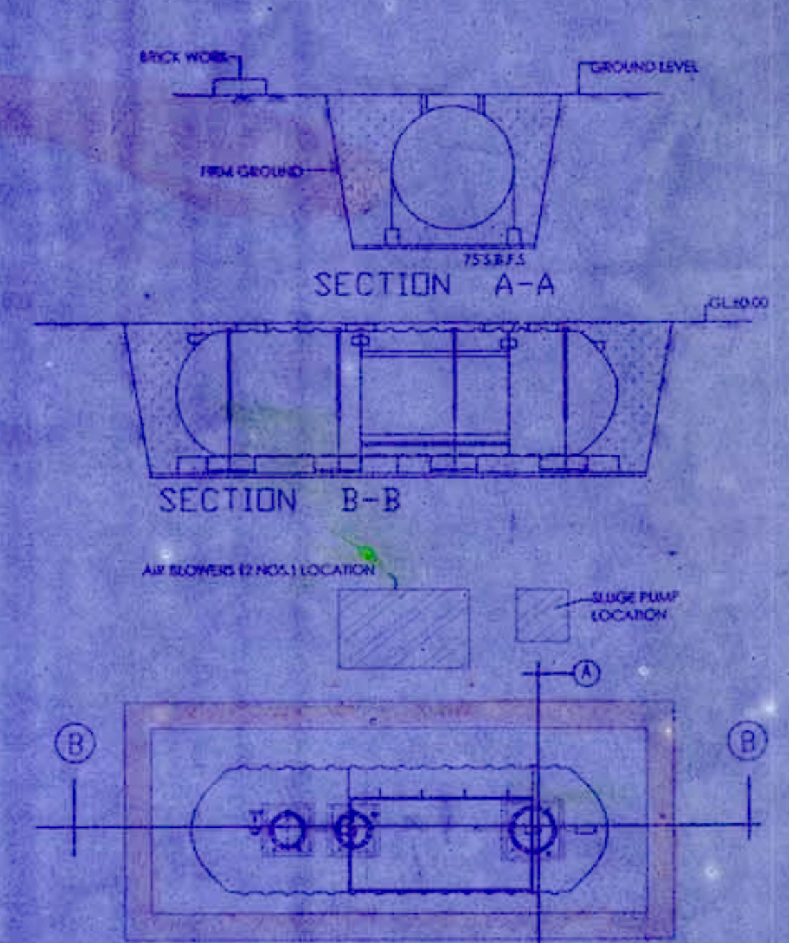
TYP. DETAILS OF S.T.P. (SCALE = 1:100) 350 USER -> STP-1 -> AREA (15M x 5M x 3M HL) 350 USER -> STP-2 -> AREA (15M x 5M x 3M HL) 250 USER -> STP-3 -> AREA (11M x 5M x 3M HL)
