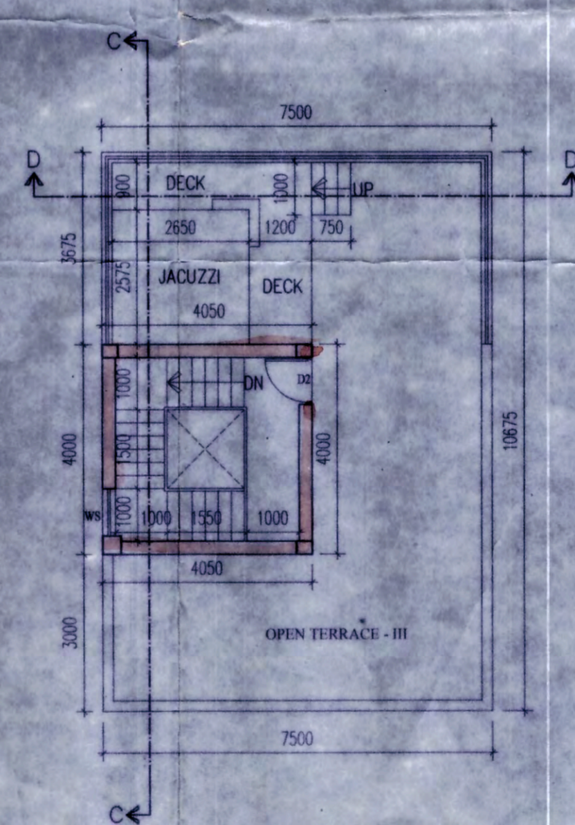
ROOF PLAN RESIDENTIAL BUNGALOW (TYPE 03) SCALE-1:100
