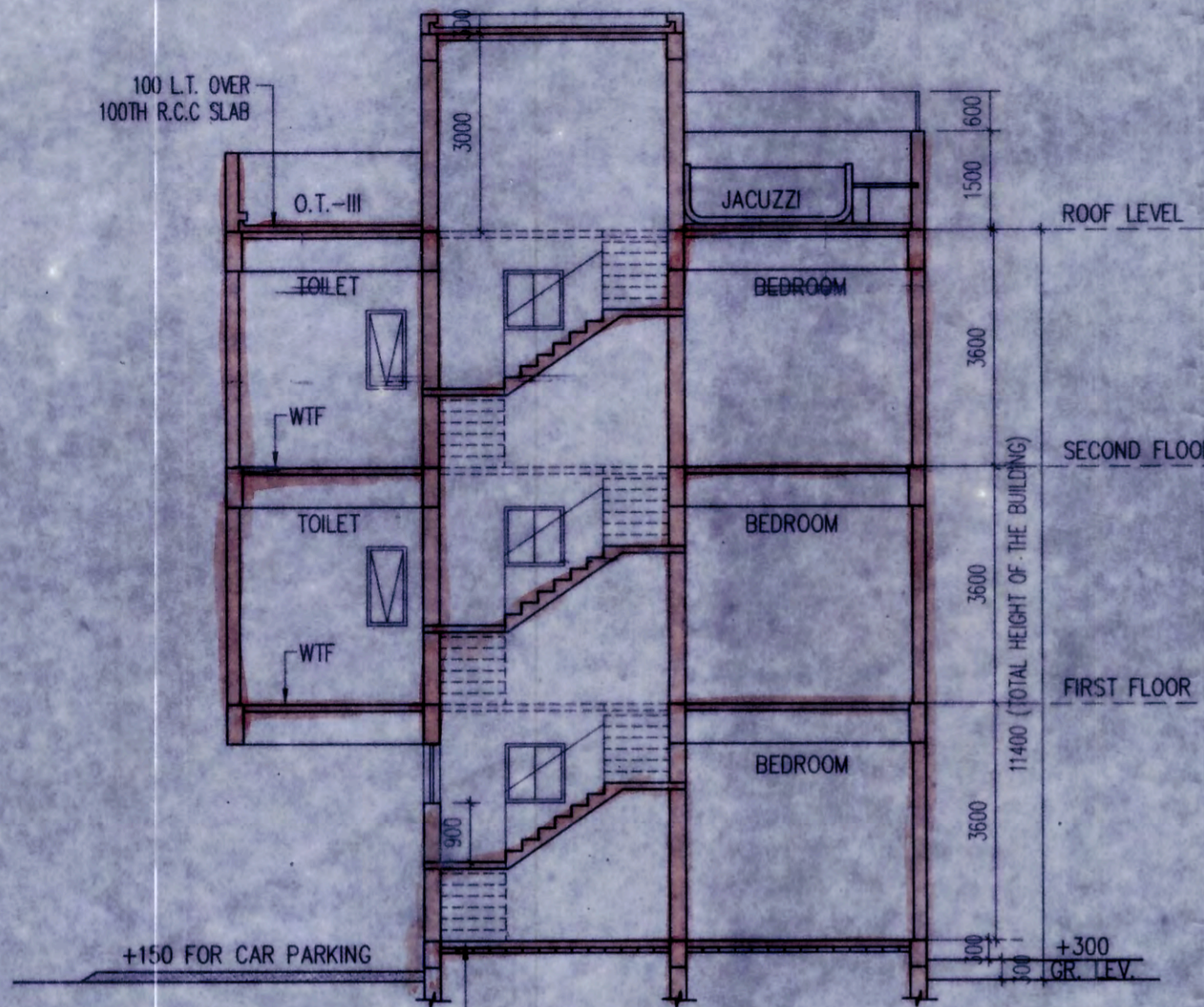
SECTION C-C
