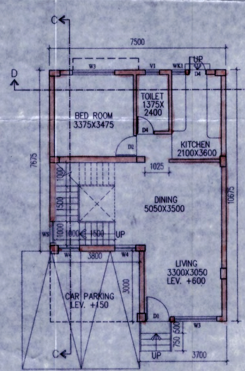
GROUND FLOOR PLAN RESIDENTIAL BUNGALOW (TYPE 03) SCALE-1:100
