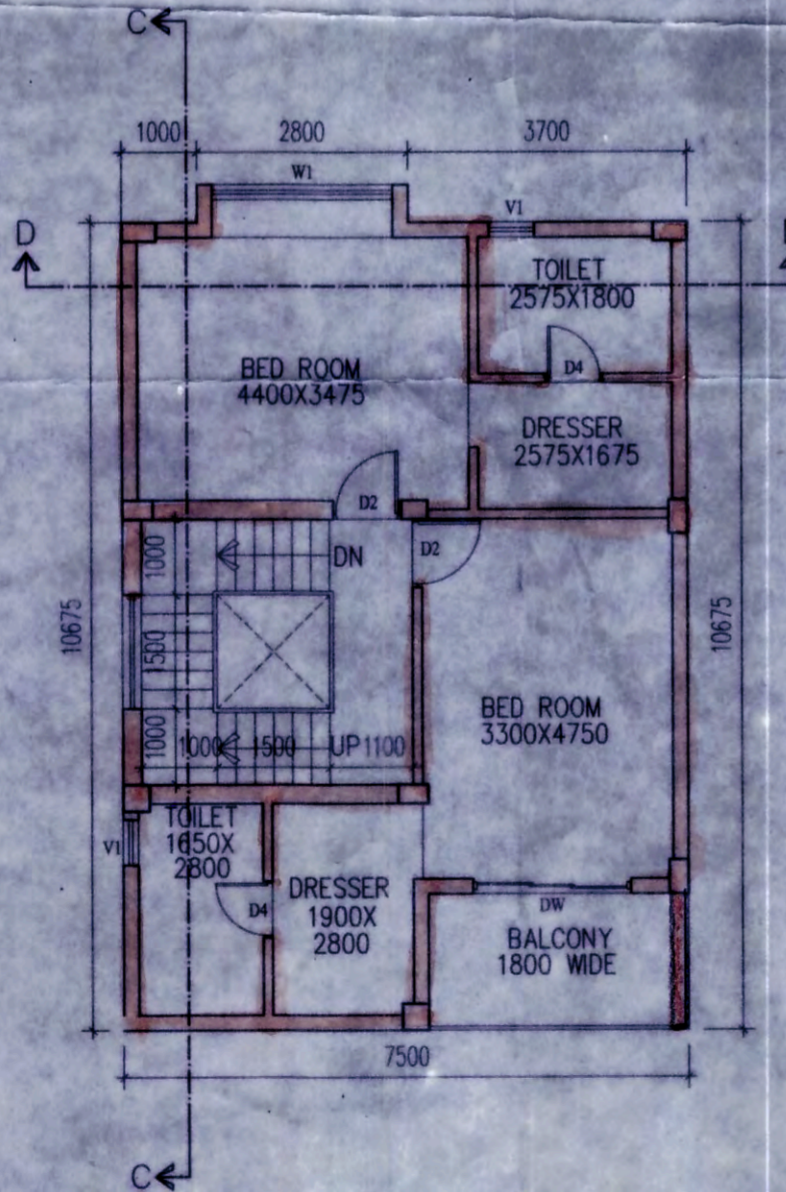
1ST & 2ND FLOOR PLAN (TYPICAL FLOOR PLAN) RESIDENTIAL BUNGALOW (TYPE 03) SCALE-1:100
