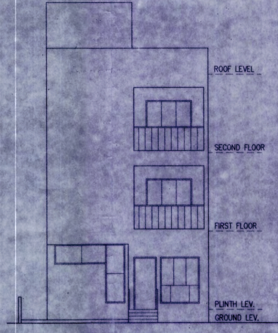
FRONT ELEVATION
