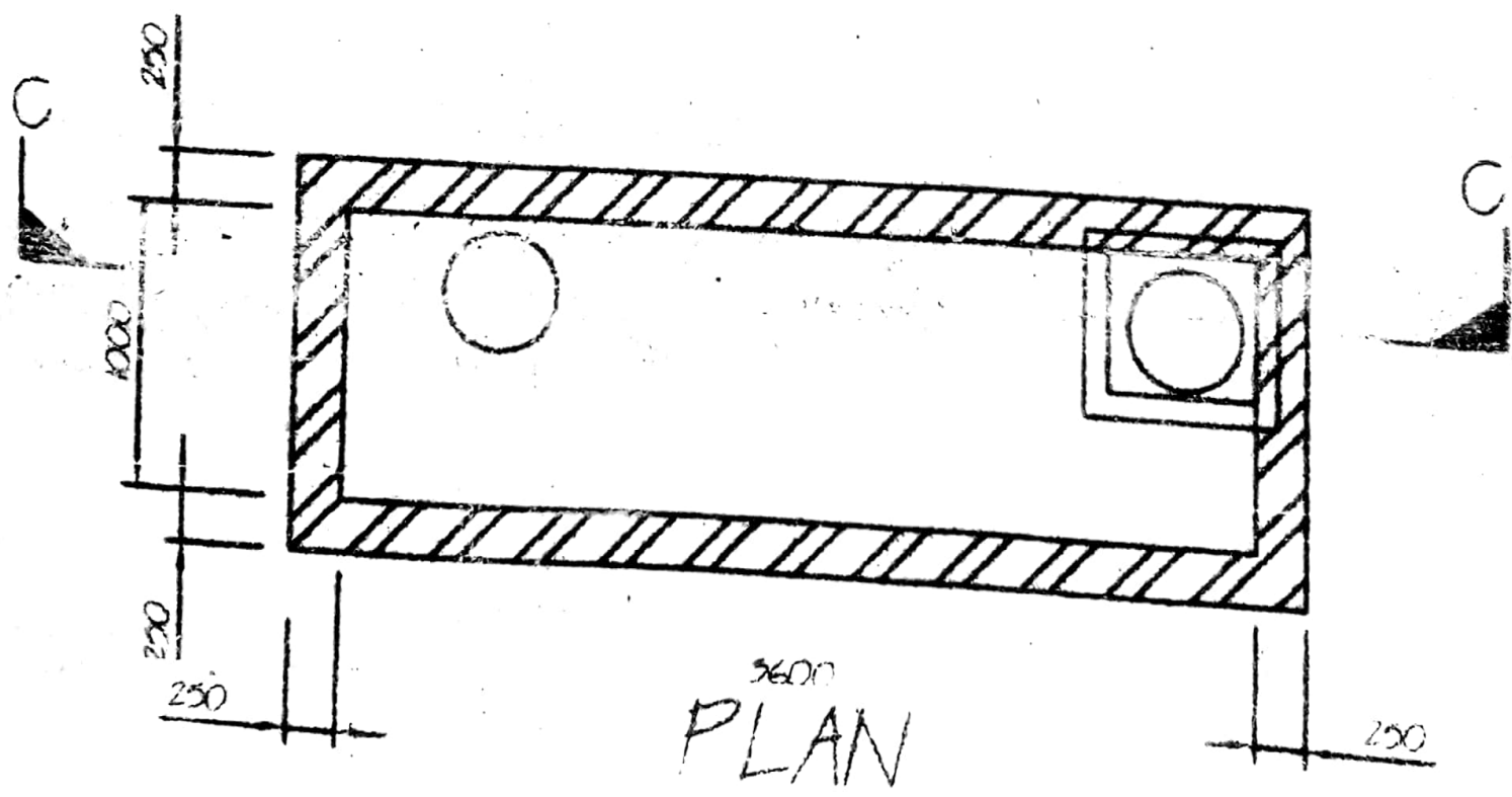
RESERVOIR (2700 LTR.) DETAIL OF SEMI U/G
