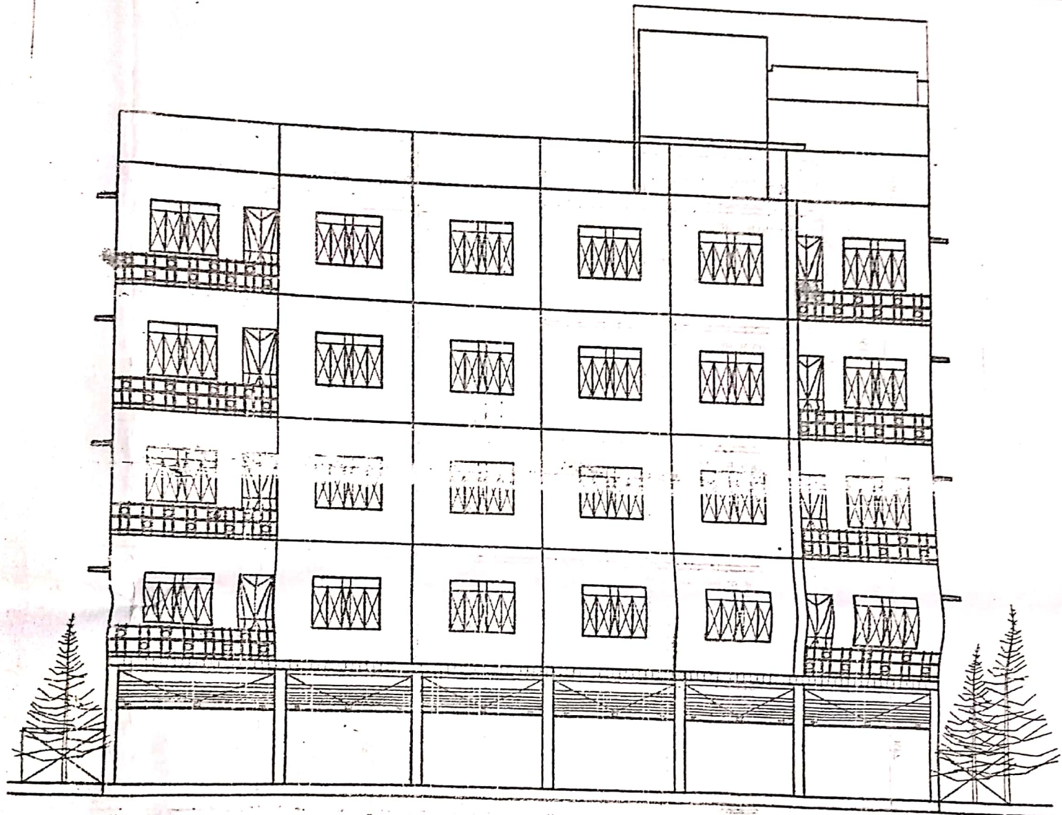
FRONT ELEVATION
