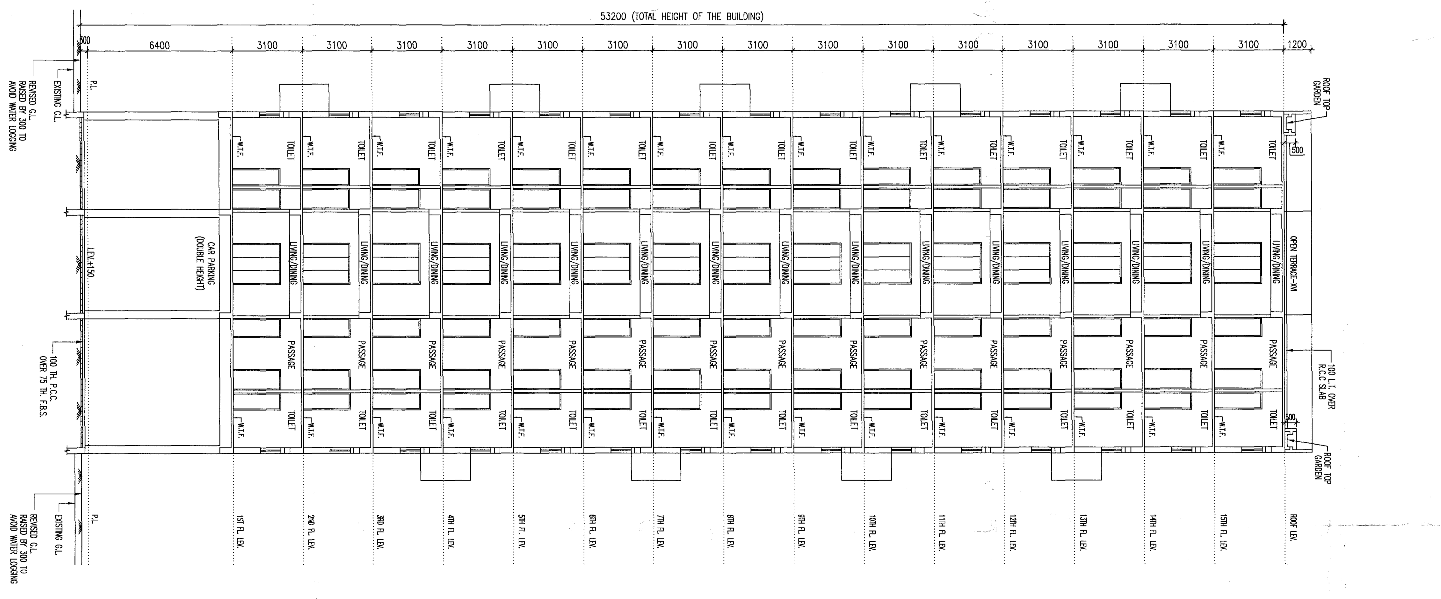
BLOCK-1 SECTION AT - BB SCALE 1:100
