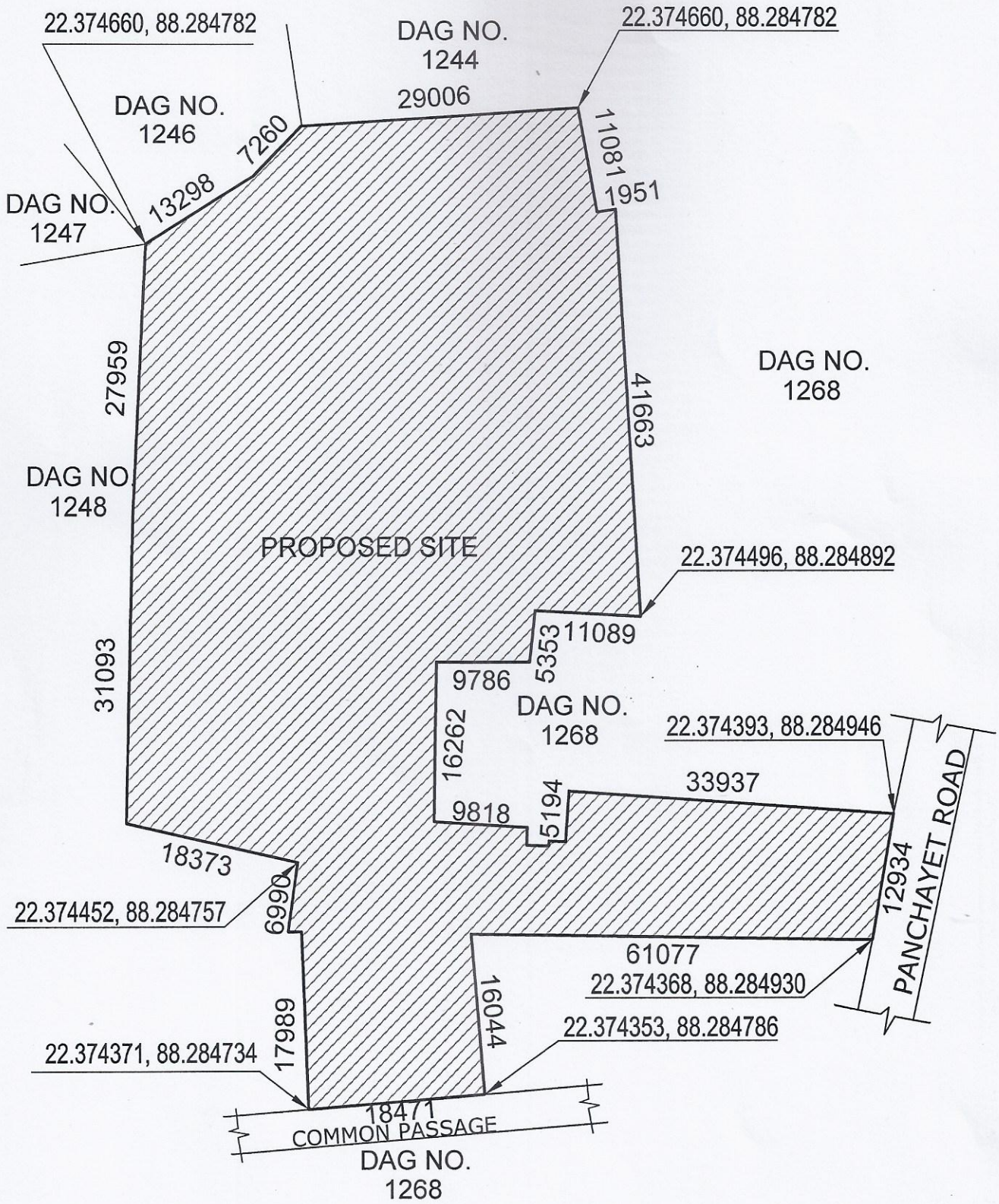
LOCATION PLAN
